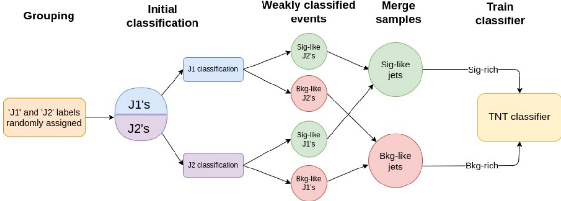
Figure A.1: A flowchart outlining how the samples for the weakly supervised training were constructed in the TNT method. The two jets in the dijet candidate were randomly assigned labels J1 and J2. For each event, the J1 (J2) jet is placed into either a signal-like or background-like sample based on the autoencoder scores evaluated on the J2 (J1) jet. The samples of signal-like (background-like) J1's and signal-like (background-like) J2's were merged together to construct a single sample of signal-like (background-like) jets. The TNT classifier is then trained to distinguish between these two samples.
