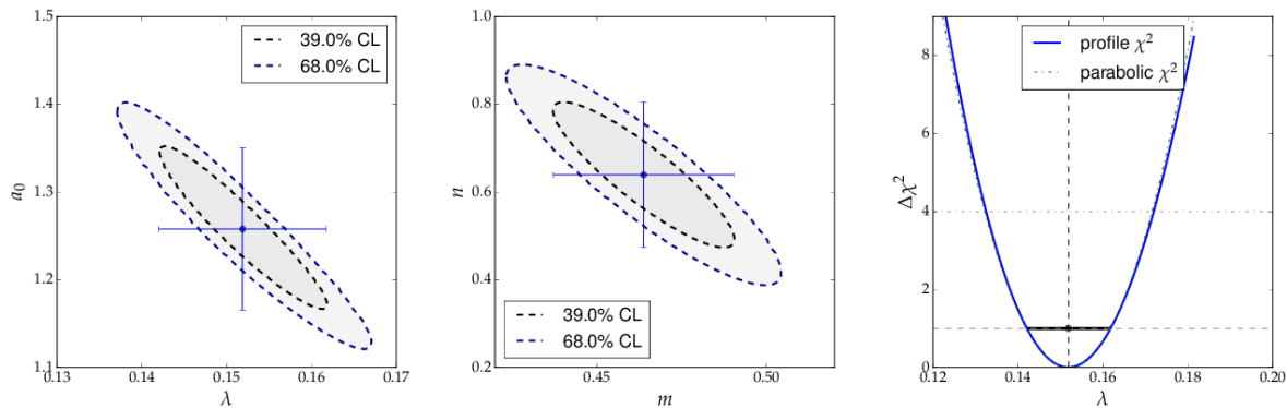
Fig. 2: Contour curves and a profile 2 curve for the fits in example 1
