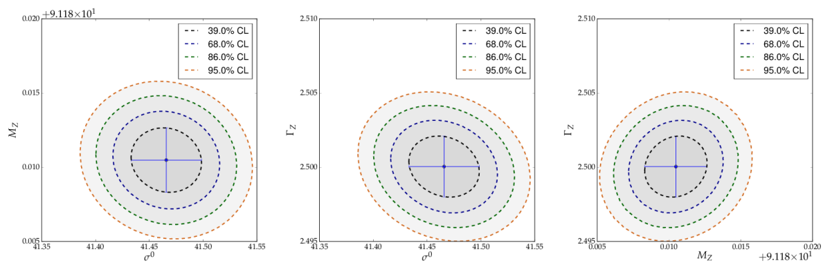
Fig. 11: Contours generated in example 8 - Fit of a Breit-Wigner function.
