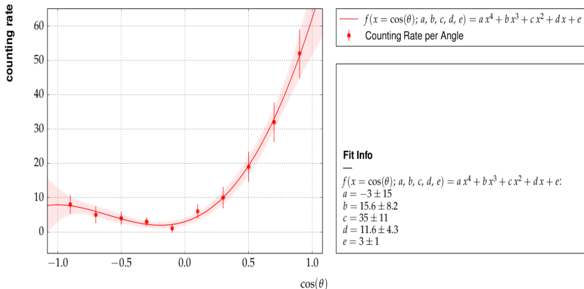
Fig. 8: Output of example 6 - counting rate.
