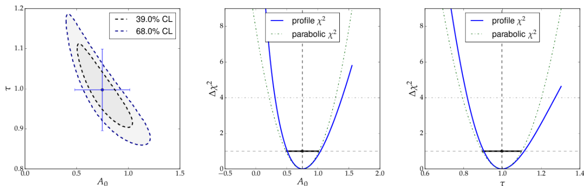
Fig. 5: Contour and profile \chi^2 curves of example 3
