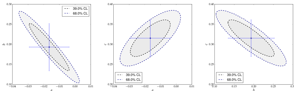
Fig. 4: Contour curves of a pairs of paramters a , b and c of the example above, calculated with kafe .
