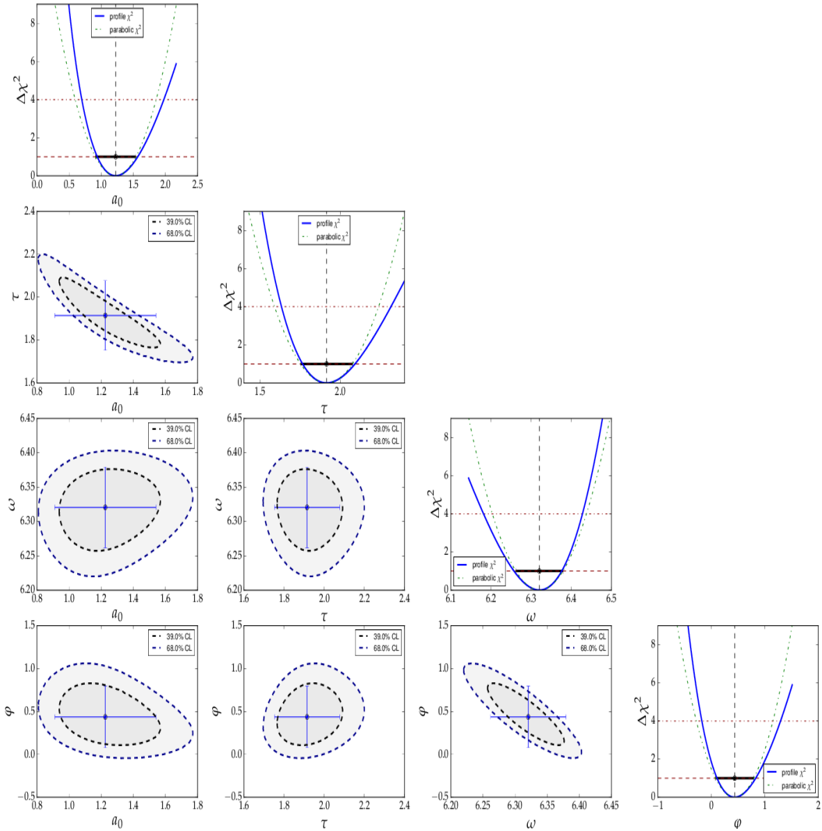
Fig. 7: Confidence contours and profiles for example 5.
