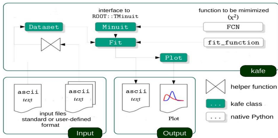
Fig. 2: Code structure of the kafe package
