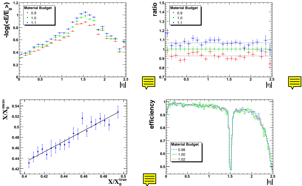
Figure 2.14: Sensitivity to variations of the tracker material budget from electron measurements based on GSF tracks; a) measured amount of material as a function of |\eta| for the nominal tracker configuration and for an integral material budget changed by \pm 10\% ; b) ratio of the measured amount of material as a function of |\eta| ; c) measured versus true thickness in X_0 of the tracker material; d) effect of a change of 2% of the material budget on the electron reconstruction efficiency.
