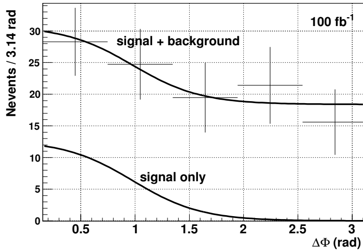
Figure 10.44: Distribution of the acoplanarity for pseudo-experiments, fitted by a signal+background shape, as described in the text.
