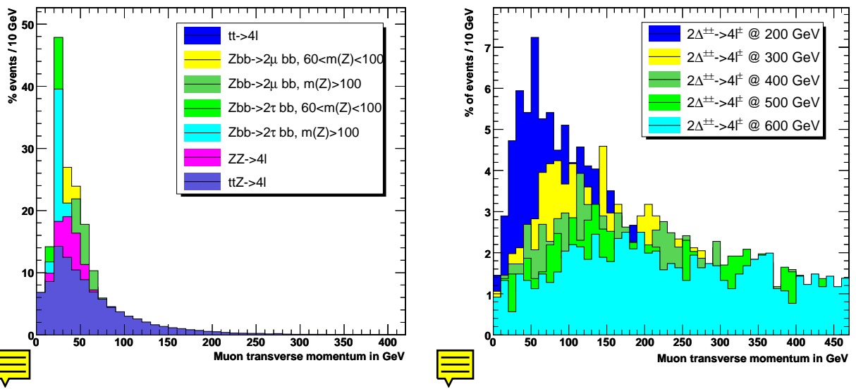
Figure 12.7: Distribution of \mu transverse momentum for background (left) and signal (right).
