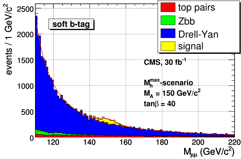
Figure 11.9: Fitting procedure applied to the di-muon reconstruction mass for the main background and for the signal sample with M_A = 150 \text{ GeV}/c^2 and \tan\beta = 40 .
