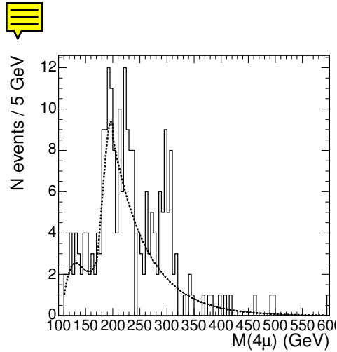
Figure A.1: The background pdf and an example of one pseudo-experiment with a statistical fluctuation appearing just like a signal.
