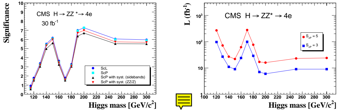
Figure 2.17: (a) Significance S_{cP} for an integrated luminosity of 30 \text{ fb}^{-1} as a function of the Higgs boson mass without and with systematics included in both options of ZZ^{(*)} normalization to the measured sidebands or the measured single Z production cross-section. The significance S_{cL} is also shown. (b) luminosity needed for a 3\sigma observation and 5\sigma discovery with the systematics included using ZZ^{(*)} normalization to the Z cross-section.
