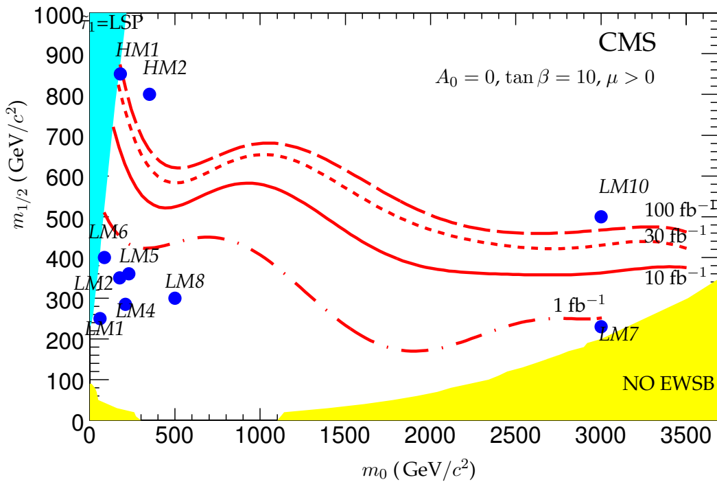
Figure 13.7: CMS reach contours (systematic uncertainties included) in the m_0 – m_{1/2} plane for SUSY processes involving two prompt same-sign muons for L = 1 \text{ fb}^{-1} (dot-dashed line), L = 10 \text{ fb}^{-1} (solid line), L = 100 \text{ fb}^{-1} (dashed line). The other mSUGRA parameters are fixed to \tan \beta = 10 , \mu > 0 and A_0 = 0 . Points corresponding to the full detector simulation and reconstruction are also shown (solid circles).
