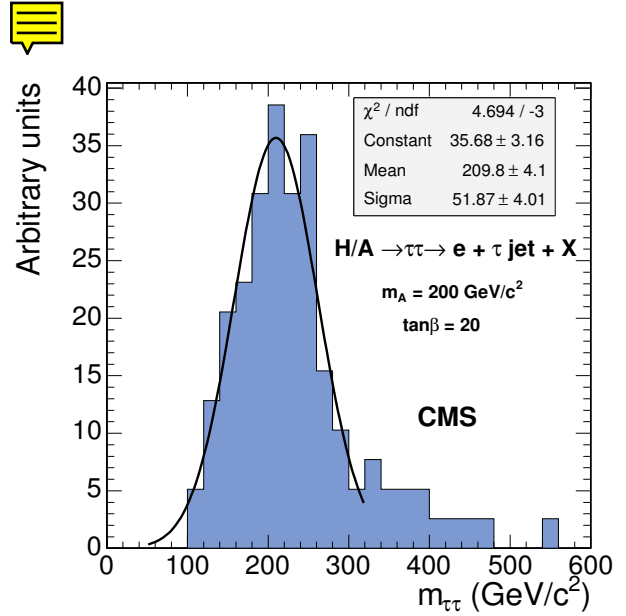
Figure 5.8: Reconstructed Higgs boson mass for m_A = 200 \text{ GeV}/c^2 and \tan\beta = 20 .
