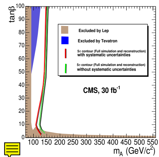
Figure 11.18: The 5\sigma contour in the (m_{A^0}, \tan\beta) plane for light charged Higgs discovery including the effect of systematic uncertainties.
