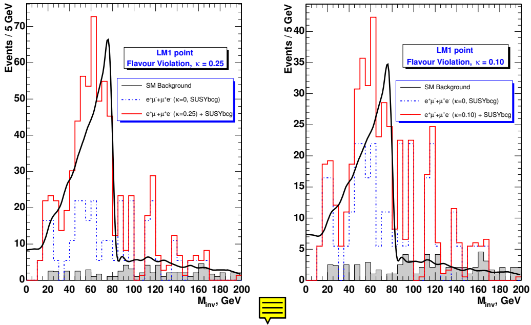
Figure 13.30: The distribution of dilepton invariant mass after selection of two isolated e^\pm \mu^\mp leptons with p_T^{lept} > 20 GeV/c and E_T^{miss} > 300 GeV for flavour violation parameter k = 0.25 (left) and k = 0.1 (right). The superimposed curves are fits to the invariant mass distribution for the case of 100% LFV.
