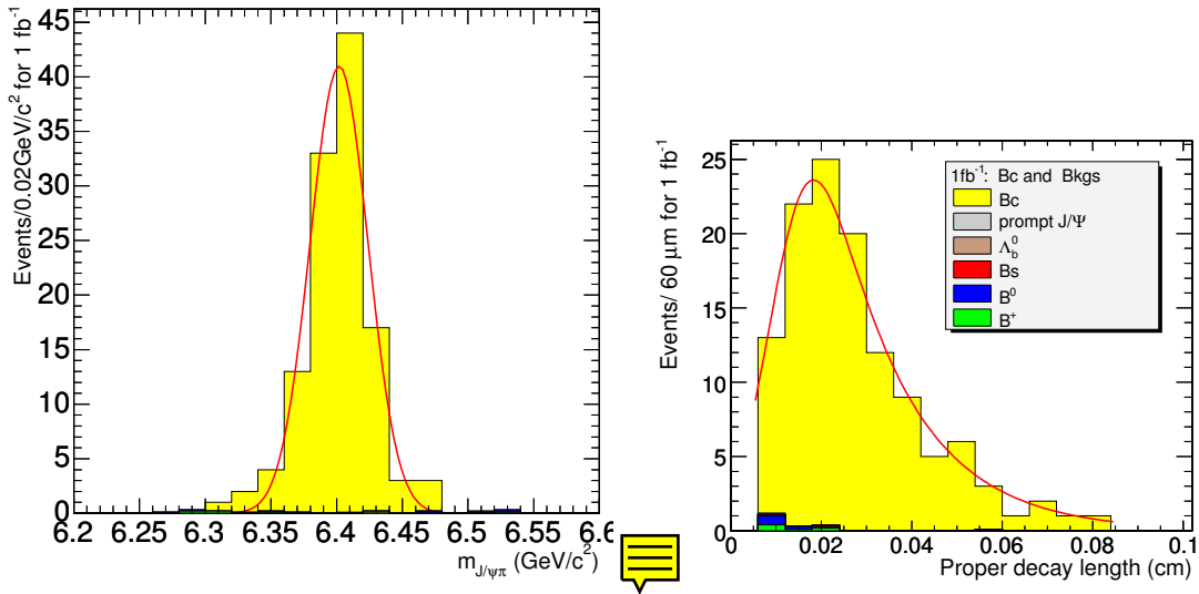
Figure 7.12: Left: The invariant mass of the J/\Psi and pion candidate for the selected B_c . Right: The B_c proper decay length distribution. Both plots correspond to 1 \text{ fb}^{-1} .
