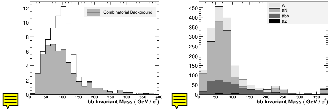
Figure 5.16: t\bar{t}H ( W \rightarrow qq' , W \rightarrow \mu\nu ). Left: Invariant b\bar{b} mass for signal only (combinatorial background is shaded grey). Right: The sum of the reconstructed m_{b\bar{b}} spectra for backgrounds with a value of L_{bSele} > 0.55 . The distributions are normalized to an integrated luminosity of 60\text{fb}^{-1} .
