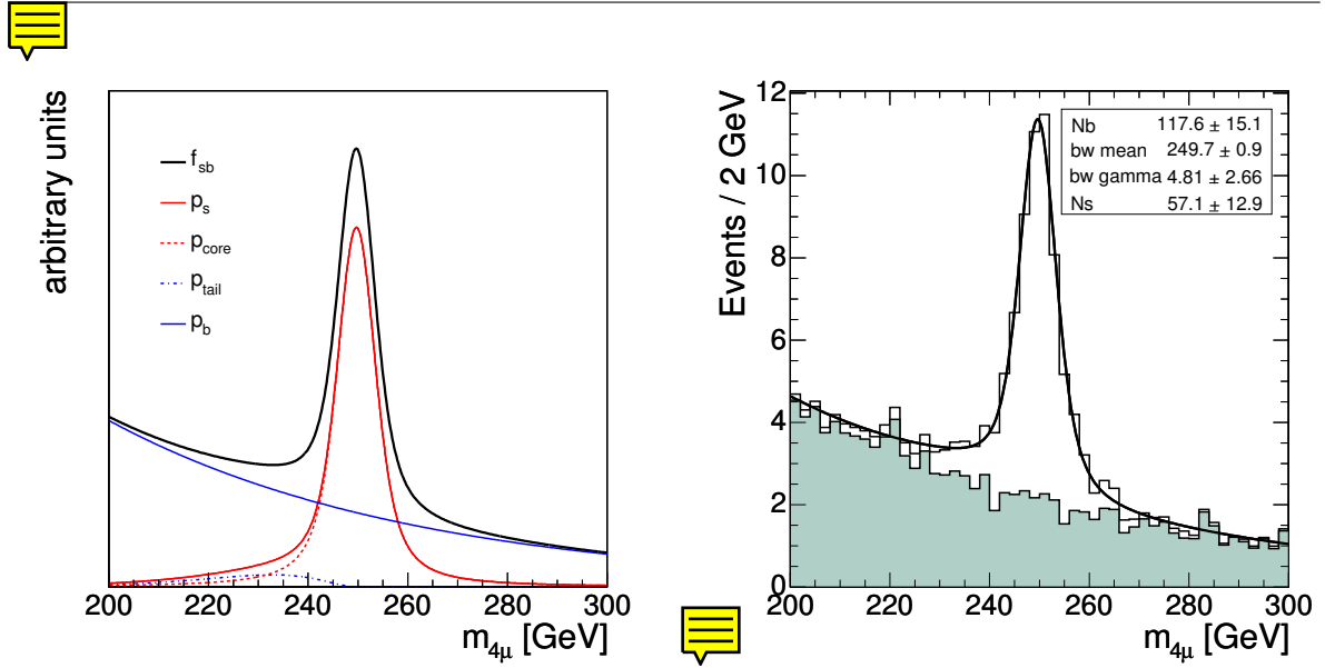
Figure 3.9: (Left) Example of the shapes of the different contributions to f_{sb} . (Right) Data-like distribution expected for a Higgs boson signals of m_H = 250 \text{ GeV} , for an integrated luminosity of 30 \text{ fb}^{-1} , together with the result of the fit (solid line) and the expected background (shaded area). This pseudo-experiment is selected randomly.
