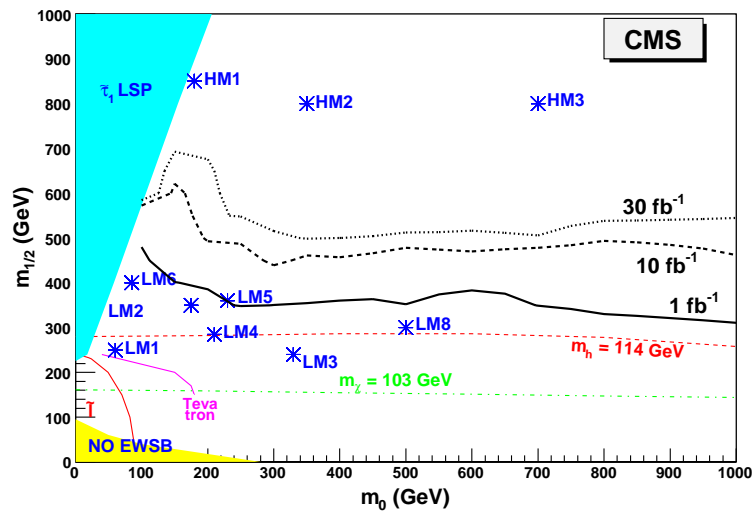
Figure 13.10: 5 \sigma discovery reach for \tan\beta = 10 , A = 0 , \mu > 0 and 1, 10, 30/fb integrated luminosity (statistical uncertainties only)
