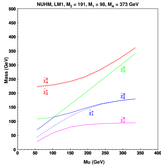
Figure 13.31: Variation of the chargino and neutralino masses as a function of \mu for the CMS test point LM1.
