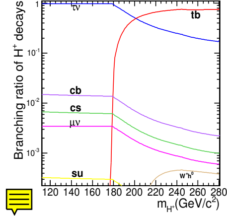
Figure 11.16: Branching ratio of charged Higgs decay to different final states for \tan\beta = 20 .
