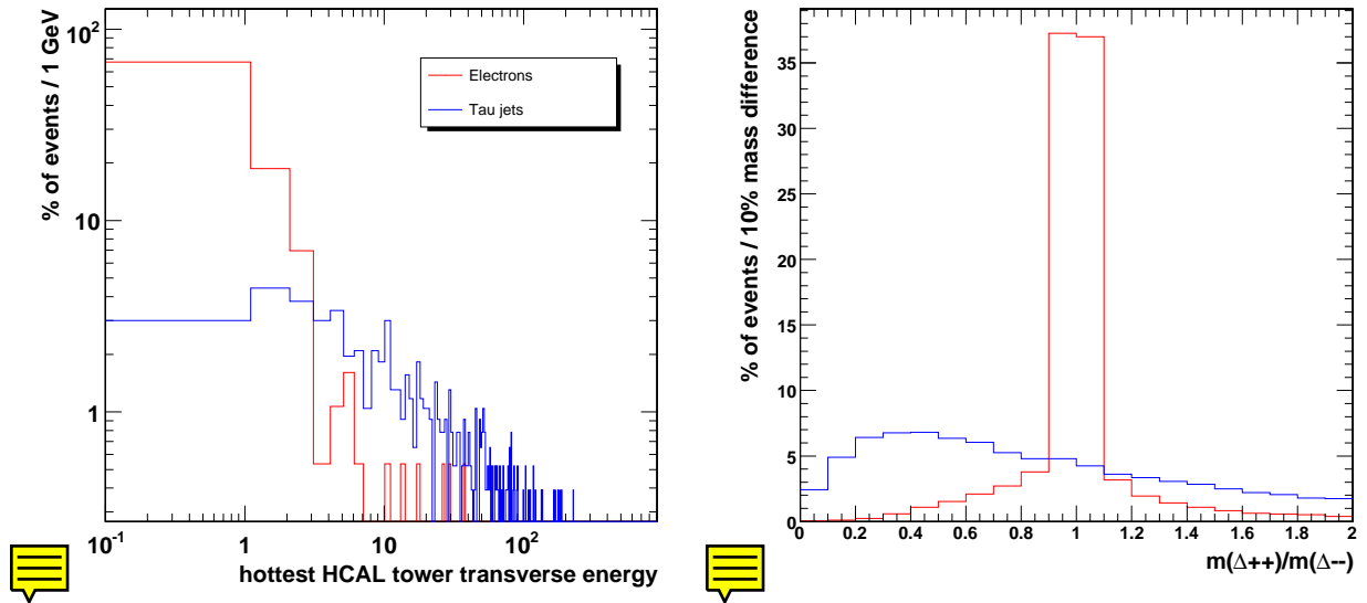
Figure 12.8: Left: Distribution of hottest HCAL tower p_{\perp} for \tau -jet candidates and electrons. Right: Distribution of m(\Delta_1)/m(\Delta_2) for background and signal.
