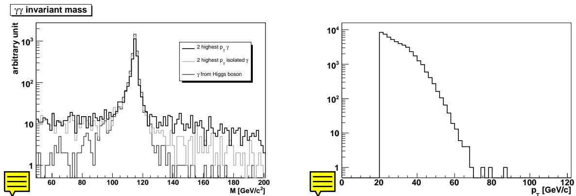
Figure 10.33: Left: Invariant mass of the two Higgs photon candidates selected according to p_T alone (dark grey curve), p_T and isolation (light grey curve), and where both candidates are geometrically matched to particle-level Higgs photons (medium grey curve). Right: Distribution of the p_T of jets from pile-up events. Jets not matched to generated particle jets from the signal are considered to be pile-up jets.
