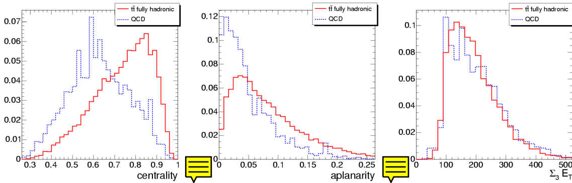
Figure 8.4: Distributions of centrality, aplanarity and \sum_3 E_T for t\bar{t} and QCD events (normalized to the same area).
