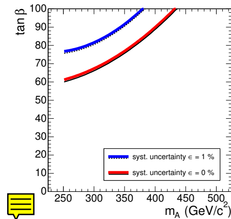
Figure 11.28: Discovery contour for the charged Higgs boson in the H^\pm \rightarrow tb decay, applying 4 b tags, for 30 \text{ fb}^{-1} ; systematic uncertainties on the background of \epsilon = 0\% , \epsilon = 1\% and \epsilon = 3\% are taken into account.
