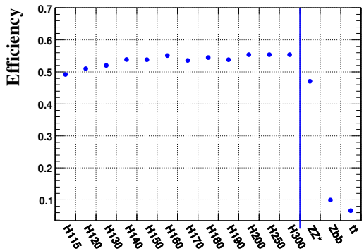
Figure 2.10: Higgs boson signal and dominant background sources after pre-selection step; a) overall pre-selection efficiency for m_H in the range from 115 to 300 \text{GeV}/c^2 and the background from ZZ^{(*)} continuum, from Zb\bar{b} and t\bar{t} ; b) separate signal and background contributions to the spectrum of reconstructed invariant mass m_{4e} .
