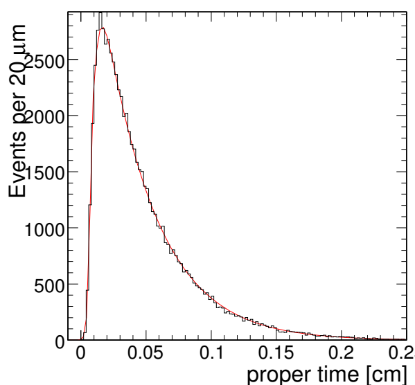
Figure 5.2: Distributions of the proper decay length of the selected signal and background events with fit projection.
