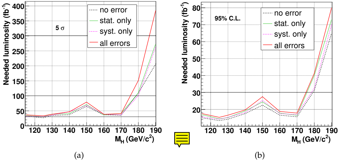
Figure 10.46: Results obtained using the benchmark fermiophobic model; (a) Luminosity needed to obtain a 5\sigma significance using the likelihood-ratio method, with systematics only, Monte-Carlo statistical uncertainties only, or with both effects considered; (b) luminosity needed to exclude a Higgs boson at 95% C.L. if no excess is observed, using the same method.
