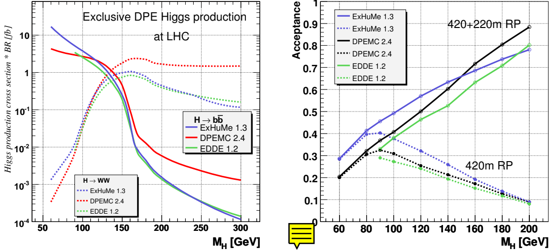
Figure 7.13: Left: The cross section for the exclusive production of the Higgs boson as a function of the Higgs boson mass for H \rightarrow b\bar{b} and H \rightarrow WW . The different curves were obtained with the generators Exhume1.3 [247], DPEMC2.4 [248] and EDDE1.2 [249]. Right: Acceptance for the 420 m detectors alone and for the combination of the 220 m and 420 m detectors as a function of the Higgs boson mass.
