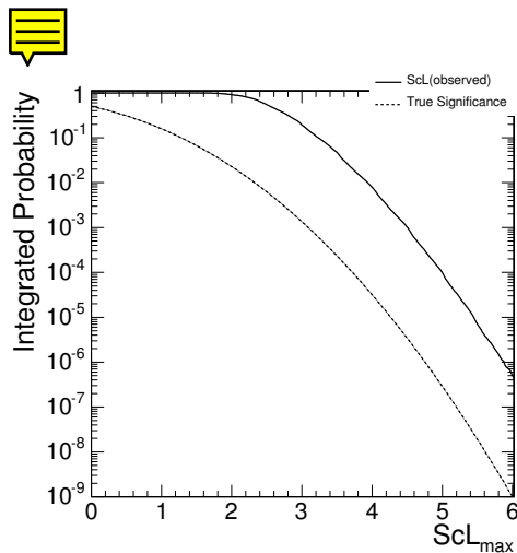
Figure A.3: S_{cL} cumulative probability density function.
