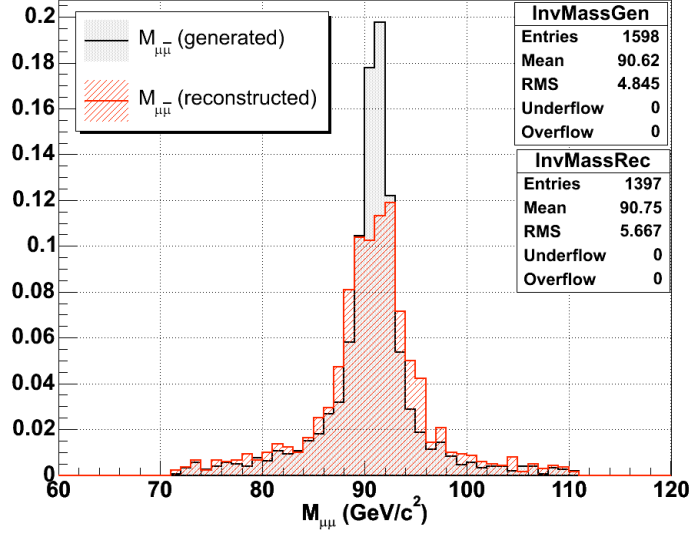
Figure 4.15: Reconstructed and generator level Z di-muon invariant mass for Z \rightarrow \mu\mu + \geq 2 jets and E_T^{miss} > 200 GeV.
