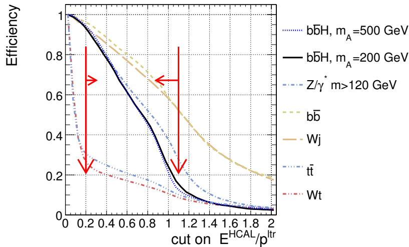
Figure 5.4: The integrated distribution of the parameter f = E^{\text{HCAL}}/p^{\text{ltr}} . The acceptance region of 0.2 < f < 1.1 is marked by the arrows (more explanations see in the text).
