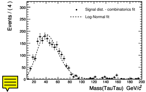
Figure 13.24: Difference between di-tau invariant mass distribution and combinatorics fit together with log-normal fit.
