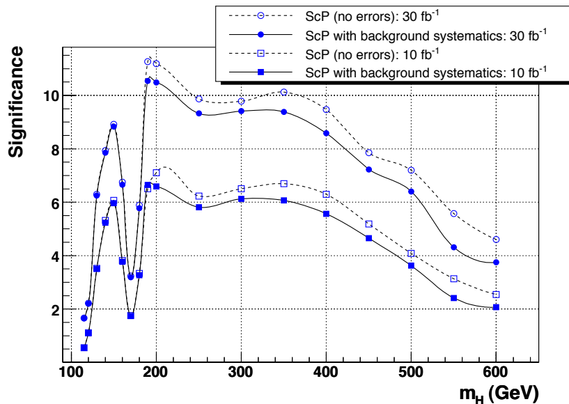
Figure 10.8: ScP significance after all selection cuts for integrated luminosities of 10\text{ fb}^{-1} and 30\text{ fb}^{-1} , with and without the systematic uncertainty on the background estimation taken into account.
