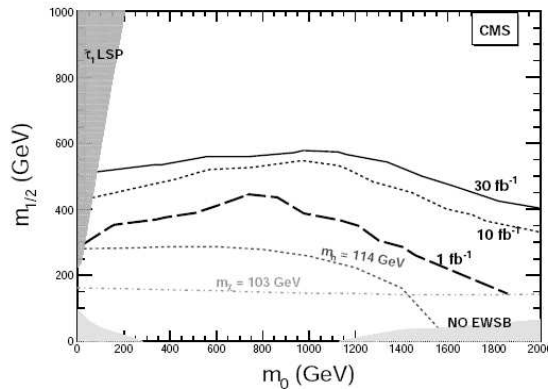
Figure 13.22: The 5\sigma reach in m_0, m_{1/2} plane with 1, 10 and 30 \text{ fb}^{-1} .
