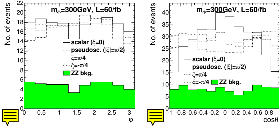
Figure 10.52: The \varphi -distributions (left) and the \theta -distributions (right) for various values of the parameter \xi after final selection (normalized to 60 \text{ fb}^{-1} ). The signal for m_\phi=300 \text{ GeV} and \xi = 0 (scalar), \xi = -\pi/4 , \xi = +\pi/4 and |\xi| = \pi/2 (pseudoscalar), respectively (empty histograms). The ZZ background - filled-up histogram.
