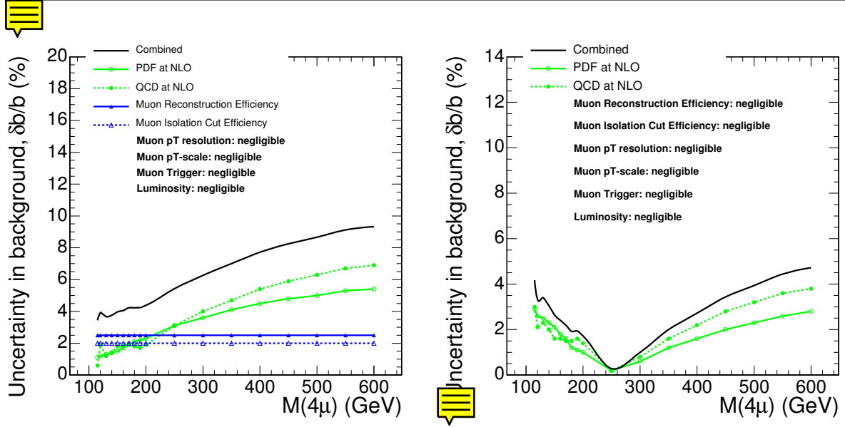
Figure 3.7: Uncertainties in the count of the ZZ \rightarrow 4\mu background events in the signal region window at different m_{4\mu} . The window size is \pm 2\sigma of the expected experimental Higgs resonance width. (Left) The background event count in the signal region is derived from the measured number of Z \rightarrow 2\mu events. (Right) The background event count in the signal region, b , is calculated from the number of ZZ \rightarrow 4\mu events B in the range 100 GeV-700 GeV (excluding the signal region window), i.e. b = \rho \cdot B .
