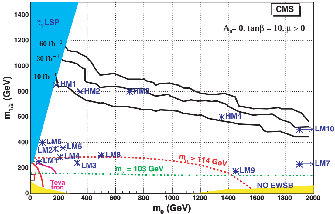
Figure 13.6: CMS discovery reach contours in the m_0 – m_{1/2} plane using inclusive muons with jets and missing energy for 10 \text{ fb}^{-1} (lower contour), 30 \text{ fb}^{-1} (middle contour), and 60 \text{ fb}^{-1} (upper contour) including systematics.
