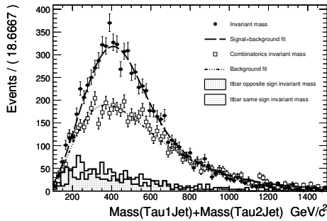
Figure 13.25: \tau_1 Jet + \tau_2 Jet invariant mass distributions.
