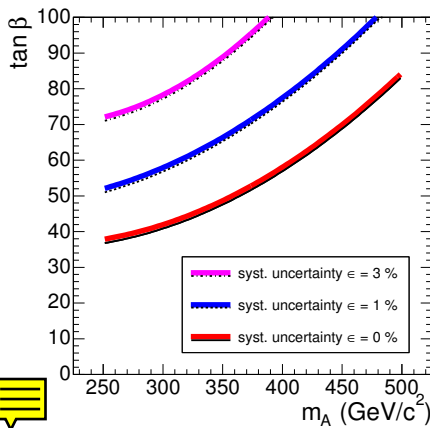
Figure 11.27: Discovery contour for the charged Higgs boson in the H^\pm \rightarrow tb decay, applying 3 b tags, for 30 \text{ fb}^{-1} ; systematic uncertainties on the background of \epsilon = 0\% , 1\% and \epsilon = 3\% are taken into account.
