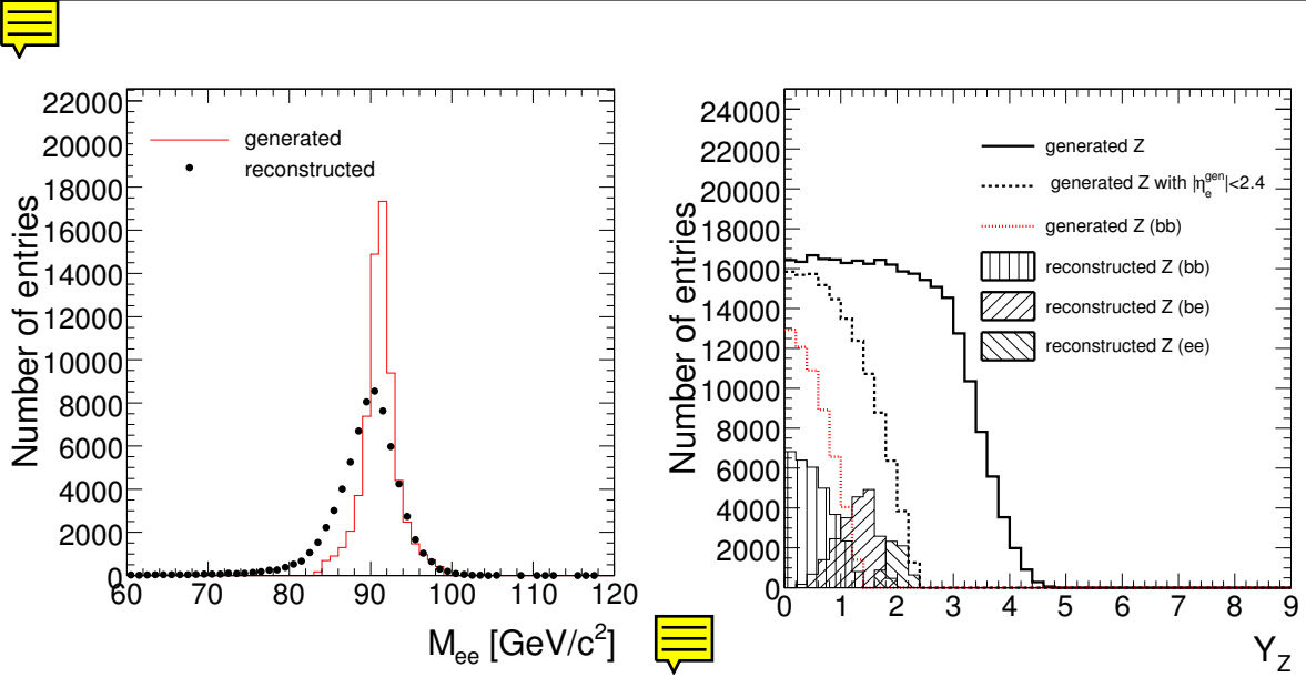
Figure 9.1: Left: Reconstructed and generated Z mass distribution with all cuts. Right: Generated rapidity distribution for all Z candidates and for those where both electrons were generated within the geometrical acceptance of the electromagnetic calorimeter. For comparison, the rapidity distribution of the finally accepted Z events is already shown here.
