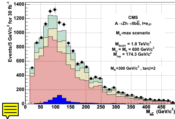
Figure 11.31: Distribution of M_{b\bar{b}} for signal and background after event selection for 30 \text{ fb}^{-1} of integrated luminosity. Red (dark gray), yellow (light gray) and green (medium gray) distributions represent the Zb\bar{b} , t\bar{t} and Z+\text{jets} backgrounds. Blue (black) distribution is the signal ( M_A=300, \tan\beta=2 ) and black dots the data (sum of the signal and the background).
