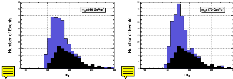
Figure 10.19: Results of VBF Higgs mass reconstruction based on signal+background (blue) and background (black)
