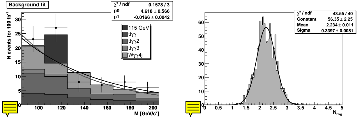
Figure 10.34: Left: Background estimation from the fit of the sidebands: Example of a gedanken experiment giving a possible set of real data points consistent with the Poisson distribution of the simulated number of surviving background events. The fit through these points is superimposed on the original fit. Right: Distribution of the estimated number of background events from the fit of the gedanken experiments.
