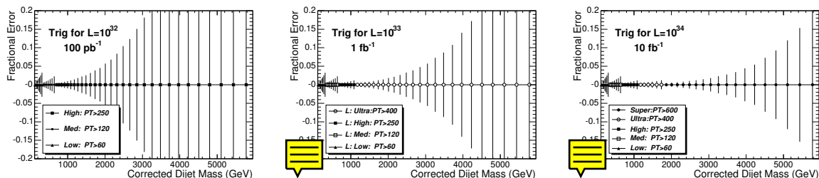
Figure 4.5: Fractional statistical error on the jet cross section for the samples in Fig. 4.5.
