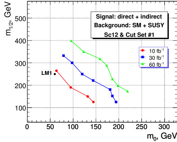
Figure 13.28: Discovery plot ( \tan\beta = 10 , \text{sign}(\mu) = + , A = 0 ) for l^+l^- .
