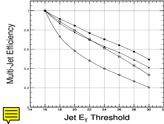
Figure 10.17: Multiple jet selection efficiency (requiring at least 4 jets in an event) as a function of jet E_T threshold. The efficiency is normalized to the rate with jet E_T threshold of 16 GeV for each sample. The physics channels include: t\bar{t} + jets (solid square), W + 3jets (open circle), W + 4 jets (solid triangle), and VBF Higgs with m_H = 170 \text{ GeV}/c^2 (open square)
