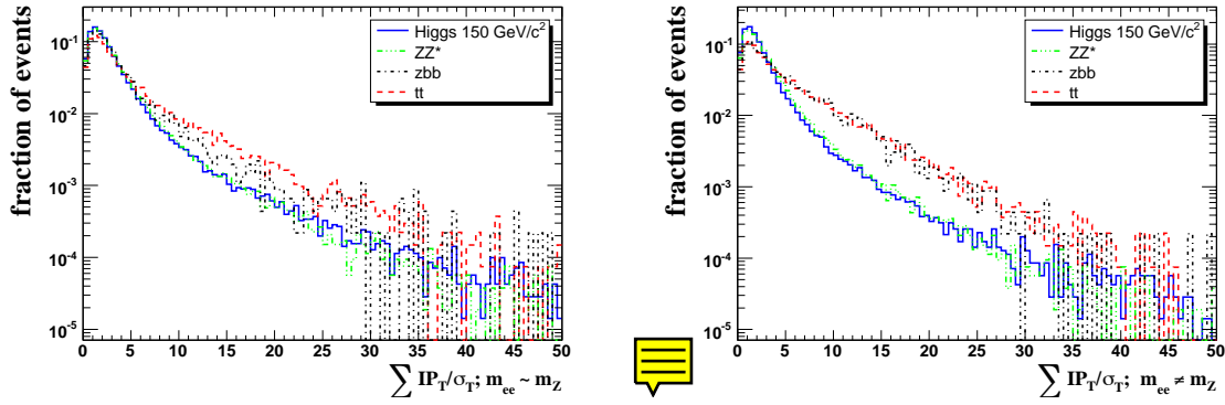
Figure 2.11: Sum of the transverse impact parameter significance ( IP_T/\sigma_T ) of e^+e^- pairs for a Higgs boson at m_H = 150 \text{ GeV}/c^2 , for the ZZ^{(*)} continuum, and for Zb\bar{b} and t\bar{t} ; a) \sum IP_T/\sigma_T from the electrons of the e^+e^- pair with a reconstructed mass m_{ee} best matching the Z boson mass; b) \sum IP_T/\sigma_T from the second (softest) e^+e^- pair.
