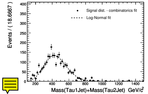
Figure 13.26: Difference between \tau_1 Jet + \tau_2 Jet invariant mass distribution and combinatorics fit together with log-normal fit.
