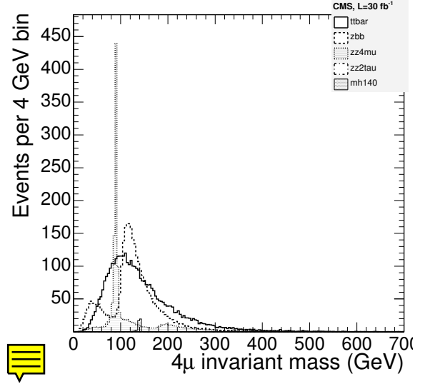
Figure 3.2: Distributions of m_{4\mu} after preselection cuts for t\bar{t} , Zb\bar{b} , ZZ and a Higgs boson signal of m_H = 140 GeV.
