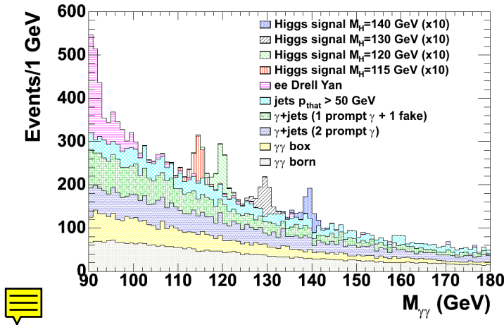
Figure 2.1: Di-photon invariant mass spectrum after the selection for the cut-based analysis. Events are normalized to an integrated luminosity of 1 \text{ fb}^{-1} and the Higgs signal, shown for different masses, is scaled by a factor 10.
