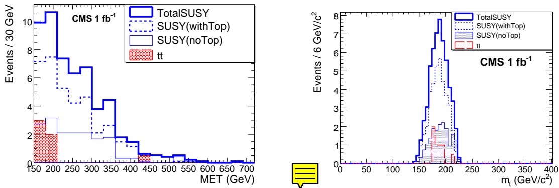
Figure 13.21: (left) Distributions of E_T^{\text{miss}} and (right) fitted top mass after all selection criteria are applied.
