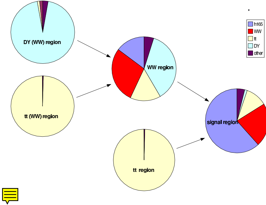
Figure 3.17: Scheme for background normalization from the data in different phase space regions: the signal region, the t\bar{t} region, the WW region, the DY (WW) region, and the t\bar{t} (WW) region. The arrows indicate the extrapolation of the number of events determined in the corresponding “control region” into the corresponding “target region”. Each region is represented by a pie chart that shows the fractions of certain types of events: h_{165} is the Higgs signal with m_h = 165 \text{ GeV} , WW is the sum of WW backgrounds, t\bar{t} is the t\bar{t} background, DY is the Drell-Yan background, and other is the sum of the Wt , ZW and ZZ backgrounds. The number of expected events in each region is reported in Tab. 3.6.
