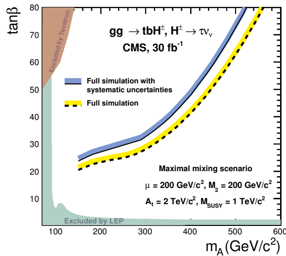
Figure 11.21: The 5\sigma -discovery region in the m_A , \tan\beta plane for gg \rightarrow tbH^\pm , H^\pm \rightarrow \tau\nu_\tau with an integrated luminosity of 30 \text{fb}^{-1} . The discovery regions with and without systematic uncertainties are shown. The regions excluded by the LEP and Tevatron searches are also shown in the figure.
