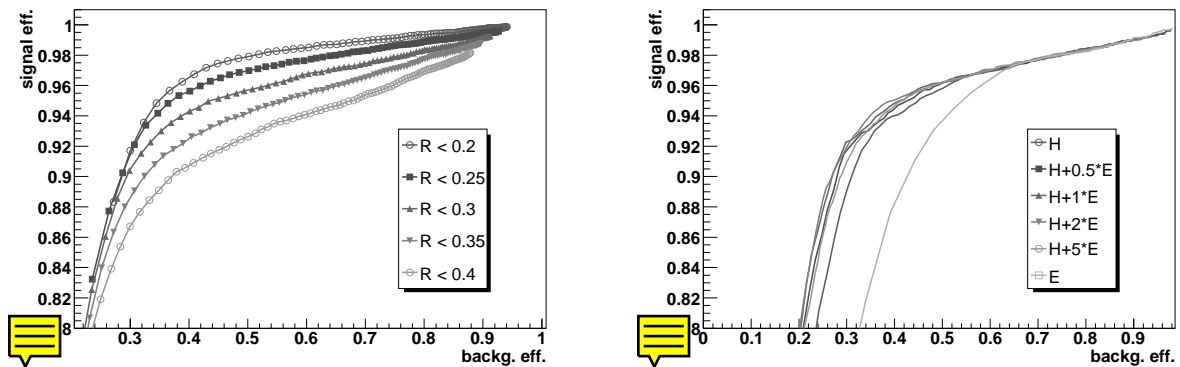
Figure 10.32: Left: Efficiency for true Higgs photons vs. that for combinatorial photons in the ECAL barrel for the ECAL isolation variable, for different isolation cone sizes. Right: Efficiency for true Higgs photons vs. that for combinatorial photons in the Ecal endcap, for several linear combinations of isolation variables.
