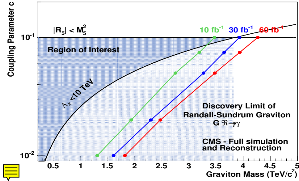
Figure 14.18: Reach of the CMS experiment in the search for the Randall-Sundrum graviton decaying into diphoton channel as a function of the coupling parameter c and the graviton mass for 10 \text{ fb}^{-1} , 30 \text{ fb}^{-1} and 60 \text{ fb}^{-1} . The left part of each curve is the region where the significance exceeds 5\sigma .
