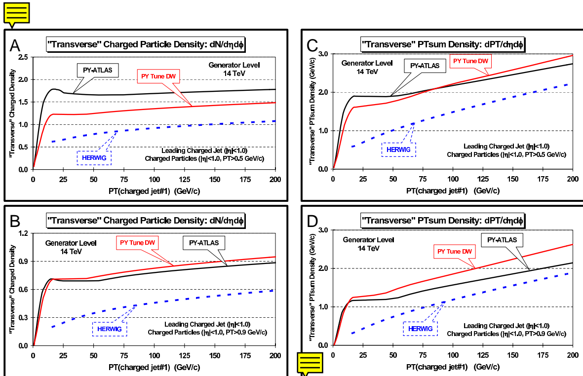
Figure 7.5: QCD Monte Carlo models predictions for charged particle jet production at 14 TeV. Left: Average density of charged particles, dN_{chg}/d\eta d\phi , with |\eta| < 1 in the “transverse” region versus the transverse momentum of the leading charged particle jet for p_T > 0.5 GeV/c (A) and p_T > 0.9 GeV/c (B). Right: Average charged PT_{sum} density, dPT_{sum}/d\eta d\phi , with |\eta| < 1 in the “transverse” region versus the transverse momentum of the leading charged particle jet for p_T > 0.5 GeV/c (C) and p_T > 0.9 GeV/c (D). The QCD models are HERWIG and two PYTHIA 6.2 tunes described in the text.
