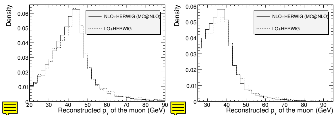
Figure 9.5: Left: Comparison between LO and NLO predictions for the muon p_T distribution in Z \rightarrow \mu\mu selected events. Both histograms have been normalized to the total number of events generated in the fiducial volume: |\eta_\mu| < 2.5 , p_{T\mu}^{max} > 20 \text{ GeV}/c , p_{T\mu}^{min} > 10 \text{ GeV}/c and M_Z - 6\Gamma_Z < M_{\mu\mu} < M_Z + 6\Gamma_Z Right: Comparison between LO and NLO predictions for the muon p_T distribution in W \rightarrow \mu\nu selected events. Both histograms have been normalized to the total number of events generated in the fiducial volume: |\eta_\mu| < 2.5 .
