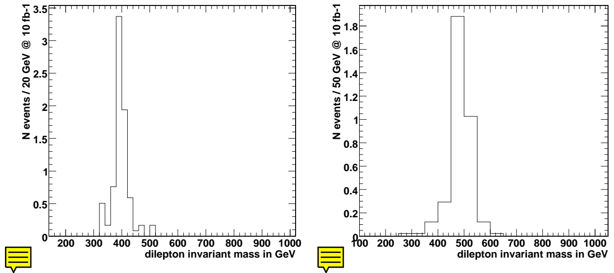
Figure 12.10: Invariant mass plots for M(\Delta^{\pm\pm})=400 GeV and 500 GeV.
