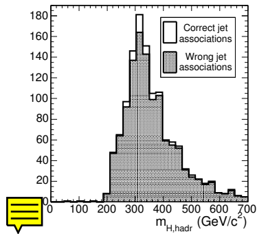
Figure 11.24: Reconstructed H^\pm mass with hadronically decaying top for the chosen jet association ( m_{H^\pm} = 311 \text{ GeV}/c^2 ).
