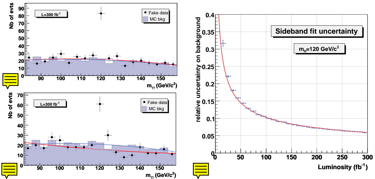
Figure 10.39: Left: Background measurement in the signal region with a fit on the m_{\gamma\gamma} sideband. The fit of the full MC statistics is represented by the solid light gray line. The fit of the fake data (dark grey) is performed on the sidebands ( i.e. after the exclusion of the signal window represented by the dotted line). Two gedanken experiments are represented for an integrated luminosity of 300 \text{ fb}^{-1} and a 120 \text{ GeV}/c^2 Higgs boson mass hypothesis. Right: Relative uncertainty on the background estimation by the sideband fit method as a function of the integrated luminosity with LHC running at high luminosity for a Higgs boson mass of 120 \text{ GeV}/c^2 .
