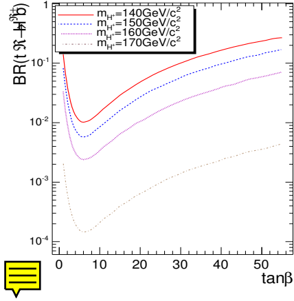
Figure 11.15: Branching ratio of top decay to H^\pm vs \tan\beta
