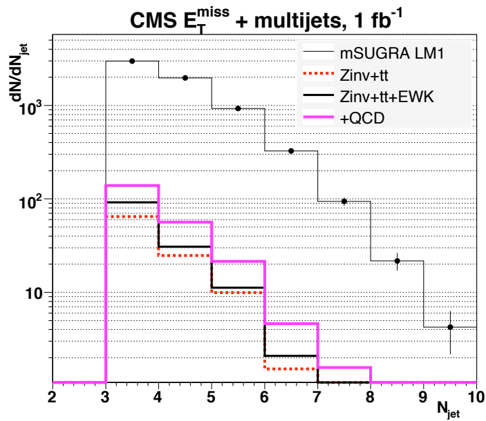
Figure 4.19: Jet Multiplicity LM1 signal and Standard Model background distributions.
