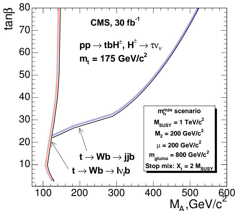
Figure 11.39: The 5\sigma discovery regions for the charged Higgs boson with the \tau\nu decay mode in the m_h^{\max} scenario.
