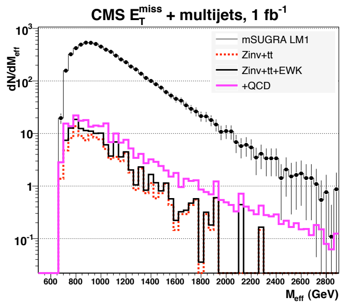
Figure 4.20: M_{\text{eff}} LM1 signal and Standard Model background distributions.
