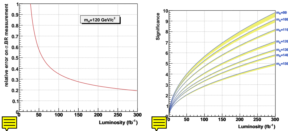
Figure 10.40: Left: Precision on the measurement of the product of cross-section and branching ratio as a function of the integrated luminosity with LHC running at high luminosity for a 120 GeV/c 2 Higgs boson. Right: Statistical significance for different Higgs boson mass hypotheses as a function of the integrated luminosity with LHC running at high luminosity. The 1\sigma systematic uncertainty is represented by the grey band.
