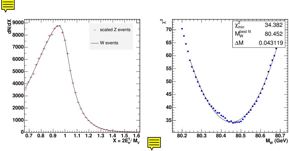
Figure 9.9: Comparison of the scaled electron E_T spectra for Z (dots) and W boson (line) events (left) and \chi^2 dependence on M_W (right) for 1 \text{ fb}^{-1} of integrated luminosity.
