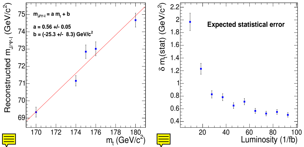
Figure 8.10: Left: correlation between the reconstructed three-lepton invariant mass and the input top mass at full simulation. Right: expected statistical error on the top quark mass as a function of the integrated luminosity.
