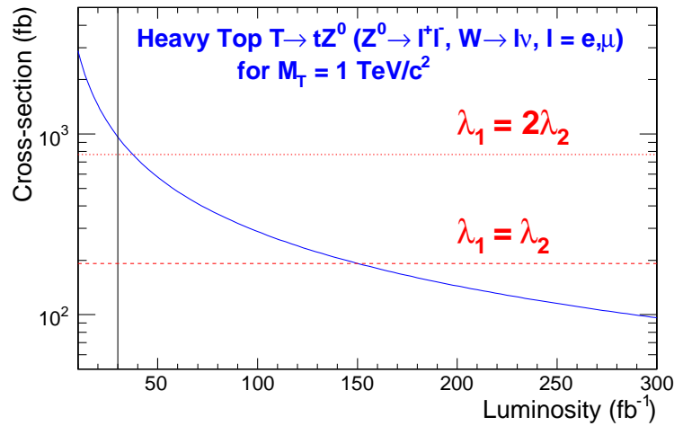
Figure 15.12: Minimum cross section for a 5 sigma discovery as a function of the luminosity for M_T = 1 \text{ TeV}/c^2 . The horizontal lines correspond to the cross section for the two values of \lambda_1/\lambda_2 .
