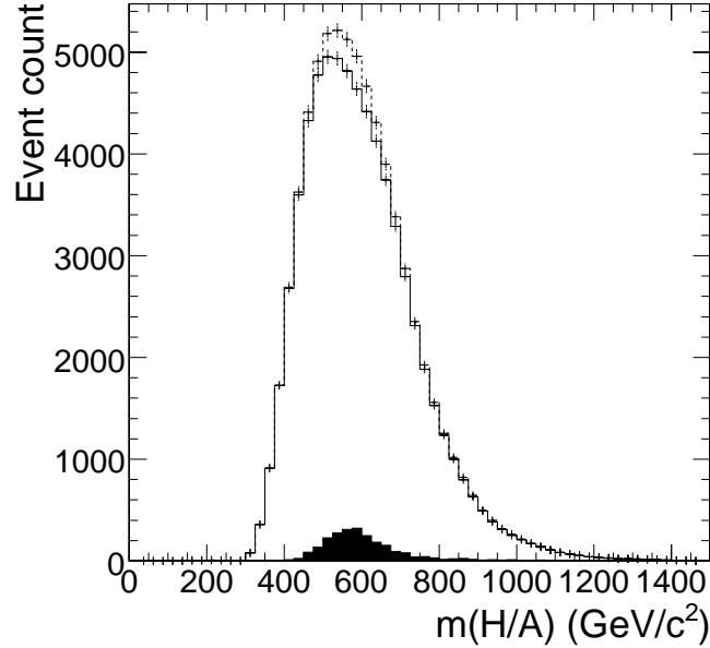
Figure 11.13: Higgs boson mass distributions after off-line and on-line selections for signal m_A = 600 \text{ GeV}/c^2 (black in foreground), background (solid line) and signal plus background (dashed line) in 60 \text{ fb}^{-1} .
