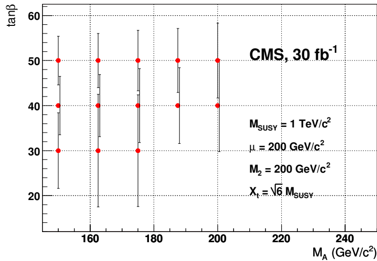
Figure 11.12: Uncertainty on the \tan\beta measurement obtained from the Higgs boson width measurement with an integrated luminosity of 30 \text{ fb}^{-1} .
