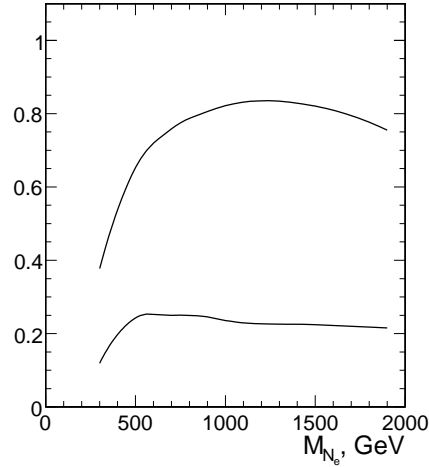
Figure 15.8: The probability to pass the primary selection for the pp \rightarrow W_R \rightarrow e + N_e \rightarrow 2e + 2jet events as a function of the N_e mass for M_{W_R} = 2 \text{ TeV}/c^2 . The lower curve is the probability to have all four W_R decay products reconstructed as separate CMS reconstruction objects
