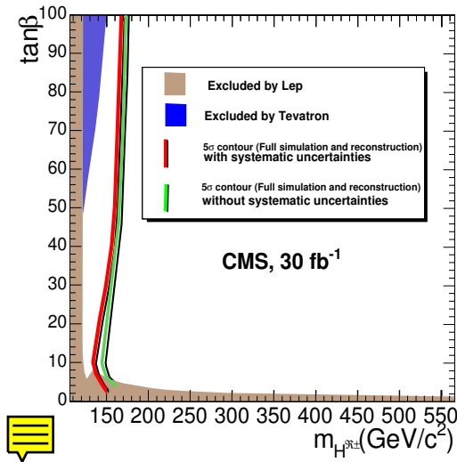
Figure 11.17: The 5\sigma contour in the (m_{H^\pm}, \tan\beta) plane for light charged Higgs discovery including the effect of systematic uncertainties.
