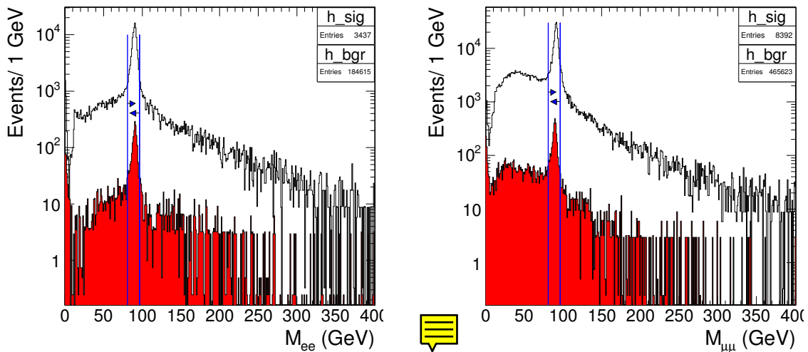
Figure 13.18: Reconstructed masses for a) e^+e^- and b) \mu^+\mu^- pairs for the background and for the signal (shaded) events. SUSY events not involving \tilde{\chi}_2^0 are considered signal. The vertical lines denote the imposed mass requirement.
