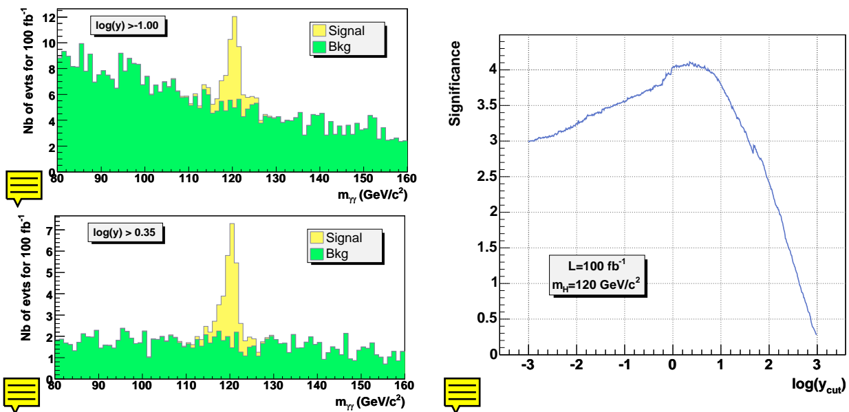
Figure 10.37: Left: Reconstructed \gamma\gamma mass for different selection values on the final combined variable y for an integrated luminosity of 100 \text{ fb}^{-1} . Right: Statistical significance as a function of the cut on the combined variable \log(y) , for m_H = 120 \text{ GeV}/c^2 and an integrated luminosity of 100 \text{ fb}^{-1} . The highest significance is obtained with a cut \log(y) > 0.35 .
