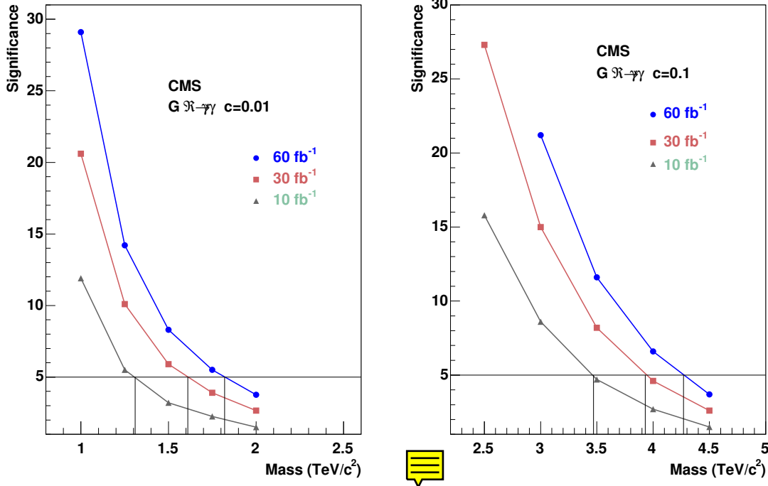
Figure 14.17: Significance as a function of the graviton mass for 10 fb^{-1} and 30 fb^{-1} integrated luminosities, c=0.01 (left) and c=0.1 (right)
