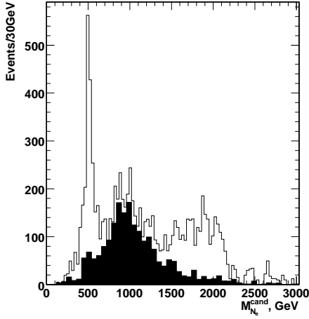
Figure 15.9: The heavy neutrino mass peak reconstructed together with the SM background (shaded histogram). The possibility to construct W_R with invariant mass above 1 TeV/ c^2 in the event is required. L_t = 30 \text{ fb}^{-1}
