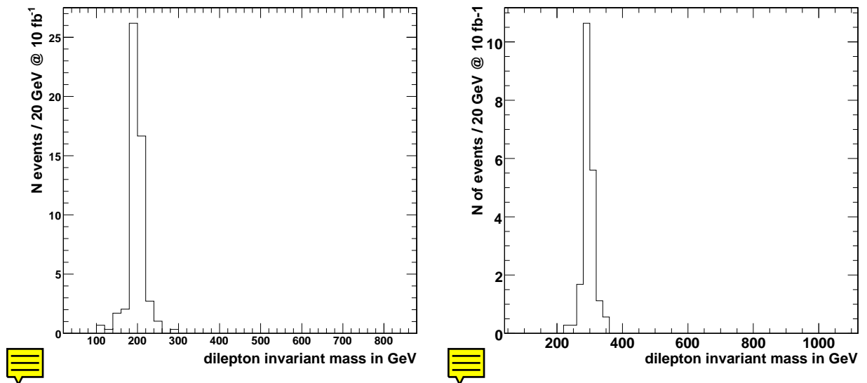
Figure 12.9: Invariant mass plots for M(\Delta^{\pm\pm})=200 GeV and 300 GeV.
