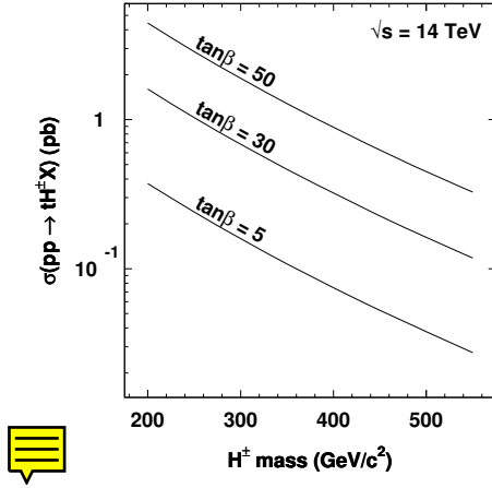
Figure 11.22: NLO cross section for pp \rightarrow tH^\pm X as a function of m_{H^\pm} .
