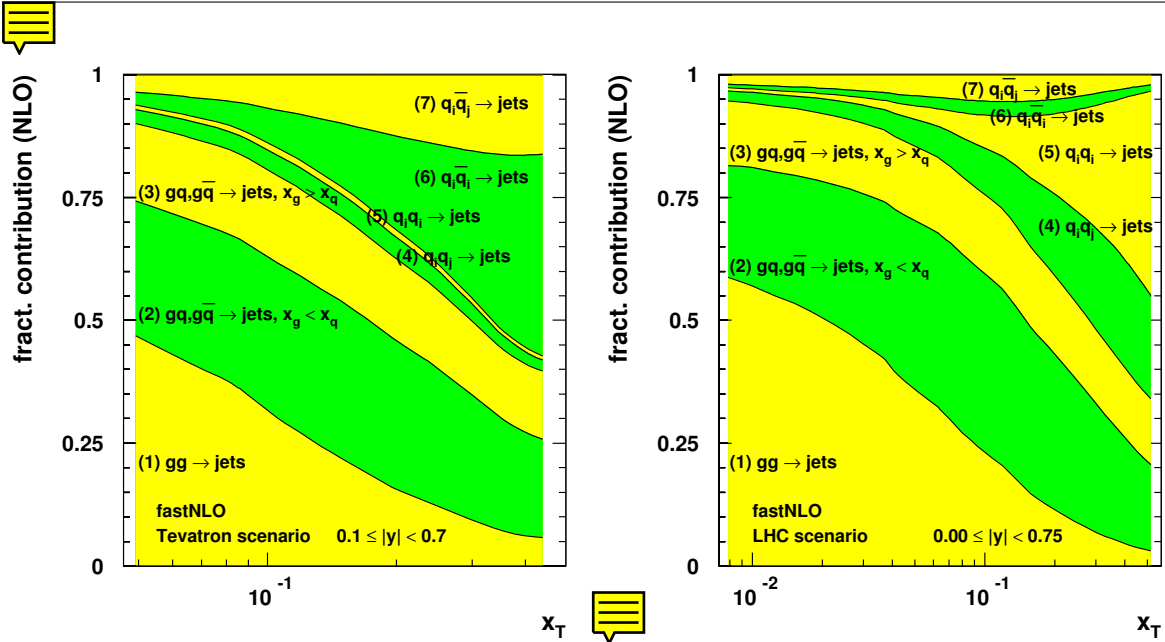
Figure 7.1: Decomposition of the total jet cross section into the partonic processes for p\bar{p} collisions at the Tevatron (left) and pp collisions at the LHC (right). The fractional contributions shown versus the scaling variable x_T = 2p_T/\sqrt{s} .
