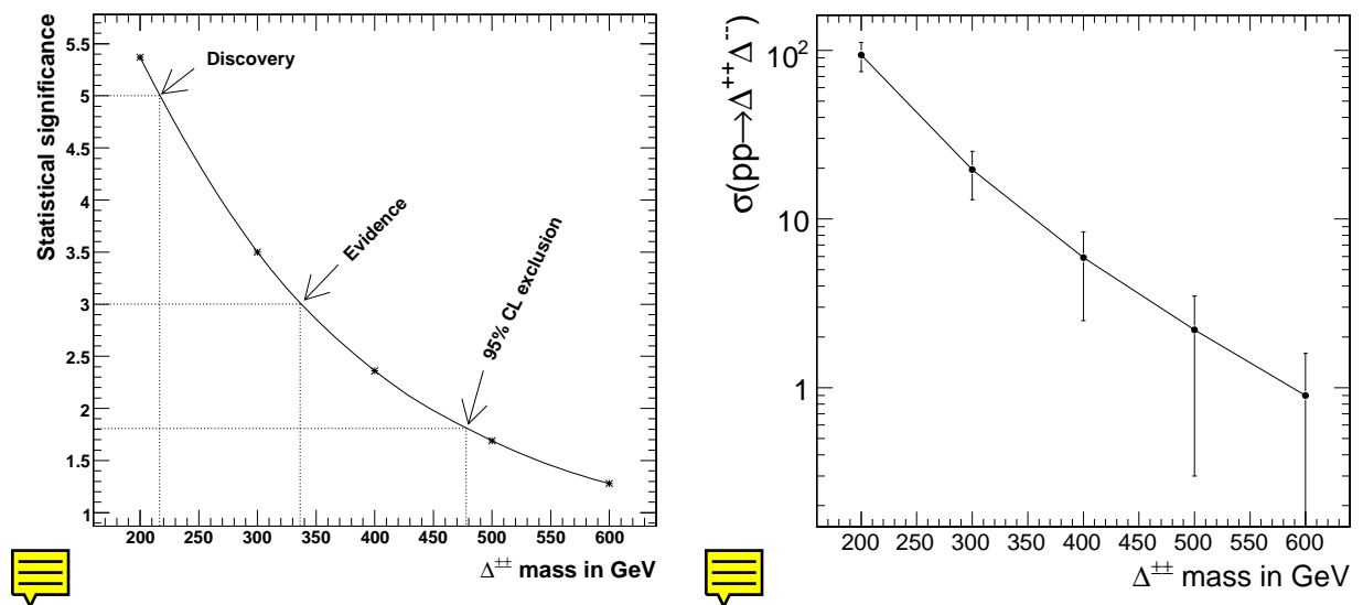
Figure 12.11: Left: statistical significance. Right: cross section with statistical errors
