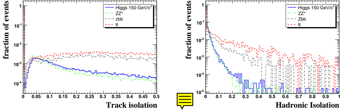
Figure 2.12: Electron isolation observables for the signal at m_H = 150 \text{ GeV}/c^2 and the SM backgrounds; a) track isolation, \sum_{\text{cone}} p_T^{\text{tracks}}/p_T^e ; b) hadronic isolation, \sum_{\text{cone}} E_T^{\text{HCAL}}/p_T^e , for the second least isolated electrons.
