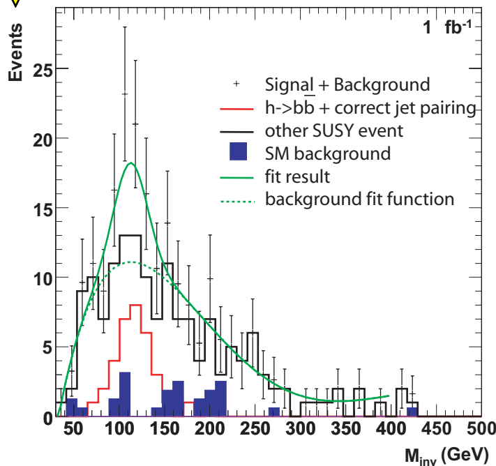
Figure 13.16: Invariant mass distribution for 1 \text{ fb}^{-1} .
