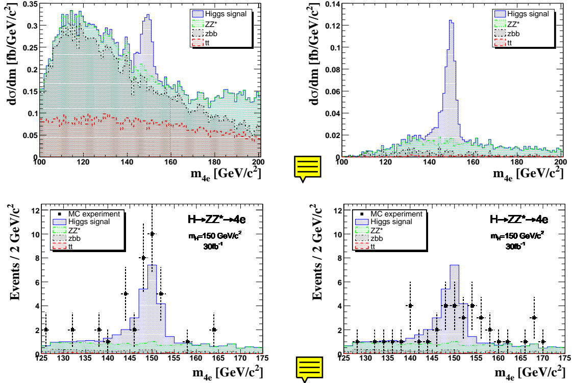
Figure 2.13: Distributions of the reconstructed invariant mass m_{4e} for the SM Higgs bosons signal at m_H = 150 \text{ GeV}/c^2 and for the SM backgrounds after (a) pre-selection step and (b) after all cuts. The number of events are normalized in cross-section. Single Monte Carlo experiments corresponding to an integrated luminosity of 30 \text{ fb}^{-1} for (c) a favorable case and (d) a less favorable case.
