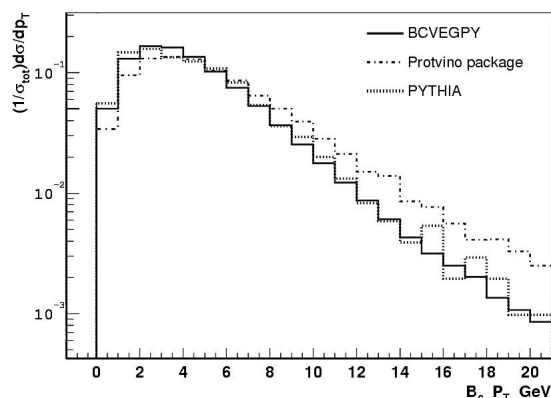
Figure 7.11: Comparison of p_T distributions of B_c mesons for the generator BCVEGPY, Gouz and PYTHIA.
