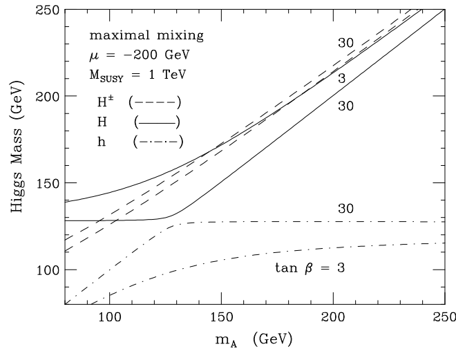
Figure 11.1: The CP-even and charged MSSM Higgs boson masses as a function of M_A for \tan \beta = 3 and 30, including radiative corrections [551].
