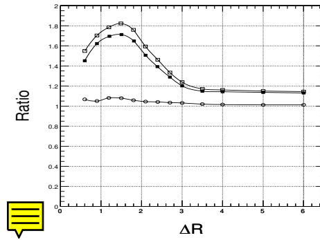
Figure 10.22: The ratio of Signal + Background Scenario to Background Only Scenario as a function of \Delta R for Region A to Region B (open square), Region A to Region C (solid square), and Region B to Region C (open circle)
