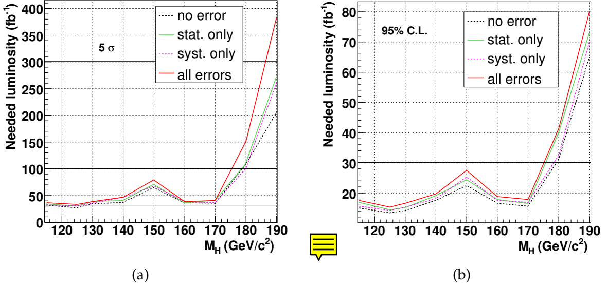
Figure 10.28: Results obtained using the benchmark fermiophobic model; (a) Luminosity needed to obtain a 5\sigma significance using the likelihood-ratio method, with systematics only, Monte-Carlo statistical uncertainties only, or with both effects considered; (b) luminosity needed to exclude a Higgs boson at 95% C.L. if no excess is observed, using the same method.
