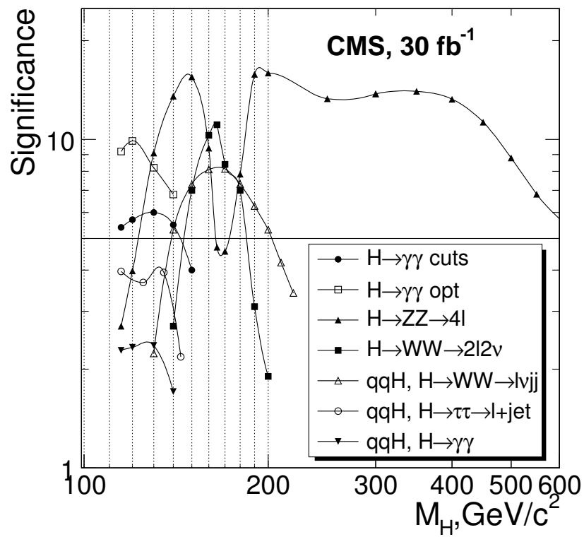
Figure 10.50: The discovery significance as a function of the Higgs boson mass for 30 \text{ fb}^{-1} of the integrated luminosity for the different Higgs boson production and decay channels
