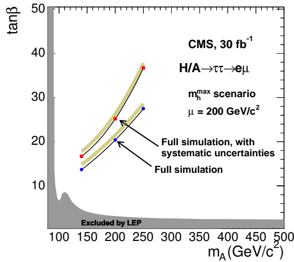
Figure 11.8: The discovery region for gg \rightarrow H/A, H/A \rightarrow \tau\tau \rightarrow e\mu + X channel in M_A - \tan\beta in the m_h^{\text{max}} scenario with 30 \text{ fb}^{-1} .
