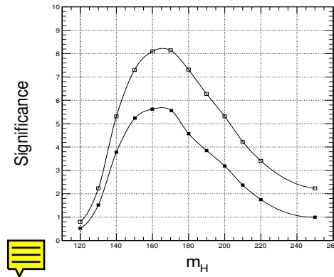
Figure 10.18: The significance of discovery potential at 30 \text{ fb}^{-1} verse Higgs boson masses. The high (low) curves of S/B and significance correspond to full (loose) extra jet veto
