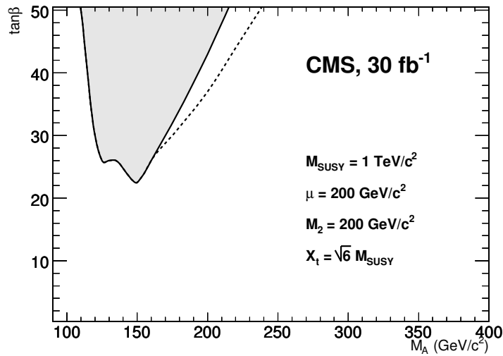
Figure 11.10: Discovery contour plot for the MSSM neutral Higgs in two muon analysis: signal points inside the grey area have a significance > 5 with an integrated luminosity of 30 \text{ fb}^{-1} . The structure of the contour plot near the minimum is due to the features of the signal in the intense coupling regime. The dashed line refers to the analysis without systematic uncertainties. It must be pointed out that the contour plot does not correspond to a significance equal to 5 for any values of M_A . In particular, for M_A < 180 \text{ GeV}/c^2 , the contour plot is actually determined by the possibility to perform a successful fit to the data, due to the low statistics. For such mass values, the contour plot corresponds to a significance which is actually slightly larger than 5. Only for M_A > 180 \text{ GeV}/c^2 the contour plot also corresponds to a significance equal to 5. This explains why the effect of the inclusion of the systematic uncertainty is visible only in this mass range. For M_A < 180 \text{ GeV}/c^2 , the fit fails even if systematic uncertainties are not included in the analysis, and the contour plot does not change.
