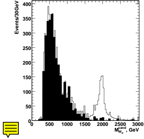
Figure 15.10: The W_R mass peak reconstructed together with the SM background (shaded histogram). L_t = 30 \text{ fb}^{-1}
