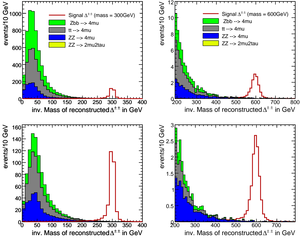
Figure 12.5: Invariant reconstructed \Delta^{\pm\pm} mass, (top) after preselection and trigger selection, (bottom) after offline cuts
