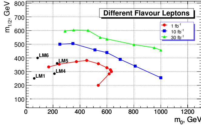
Figure 13.29: Discovery plot ( \tan\beta = 10 , \text{sign}(\mu) = + , A = 0 ) for the luminosities \mathcal{L} = 1, 10, 30 \text{ fb}^{-1} for the e^\pm\mu^\mp + E_T^{\text{miss}} signature.
