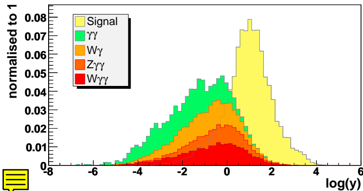
Figure 10.36: Distribution of the final combined variable for the signal ( m_H = 120 \text{ GeV}/c^2 ) and for the background. The optimal working point is obtained with a cut \log(y) > 0.35 .
