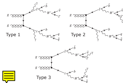
Figure 10.31: A subsample of the relative Feynman graphs illustrating the three types of t\bar{t}\gamma\gamma processes.
