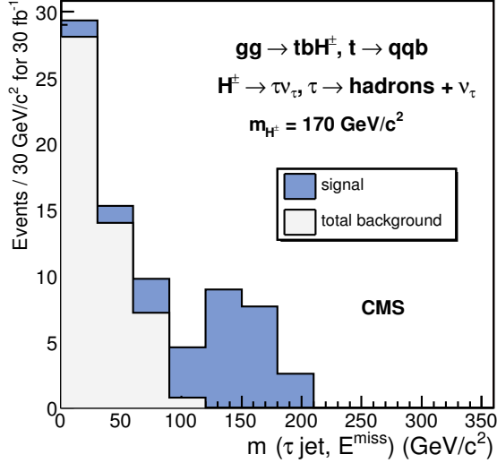
Figure 11.19: Transverse mass reconstructed from the \tau jet and missing transverse energy for the gg \rightarrow tbH^\pm, t \rightarrow bW, W^\mp \rightarrow jj signal (dark histogram) with m_{H^\pm} = 170 \text{ GeV}/c^2 , \tan\beta=30 and for the total background (light histogram) for an integrated luminosity of 30 \text{ fb}^{-1} .
