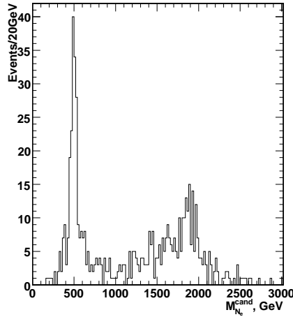
Figure 15.7: The distribution of the invariant mass M_{N_e}^{cand} for the reconstructed events with a heavy neutrino. All combinations are shown. LRRP: the simulated neutrino mass is 500 \text{GeV}/c^2 . The normalization is arbitrary.
