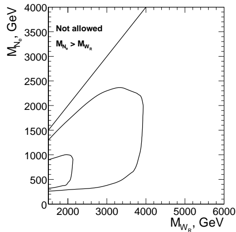
Figure 15.11: CMS discovery potential of the W_R boson and right-handed Majorana neutrinos of the Left-Right Symmetric model for the integrated luminosity L_t = 30 \text{ fb}^{-1} (outer contour) and for L_t = 1 \text{ fb}^{-1} (inner contour)
