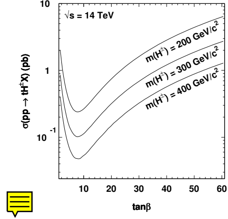
Figure 11.23: NLO cross section for pp \rightarrow tH^\pm X as a function of \tan\beta .
