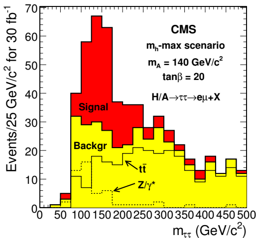
Figure 11.6: The \tau\tau reconstructed mass with 30 \text{ fb}^{-1} after all selections, but the mass window. The signal of M_A = 140 \text{ GeV}/c^2 and \tan\beta = 20 in the m_h^{\text{max}} scenario and the backgrounds are shown.
