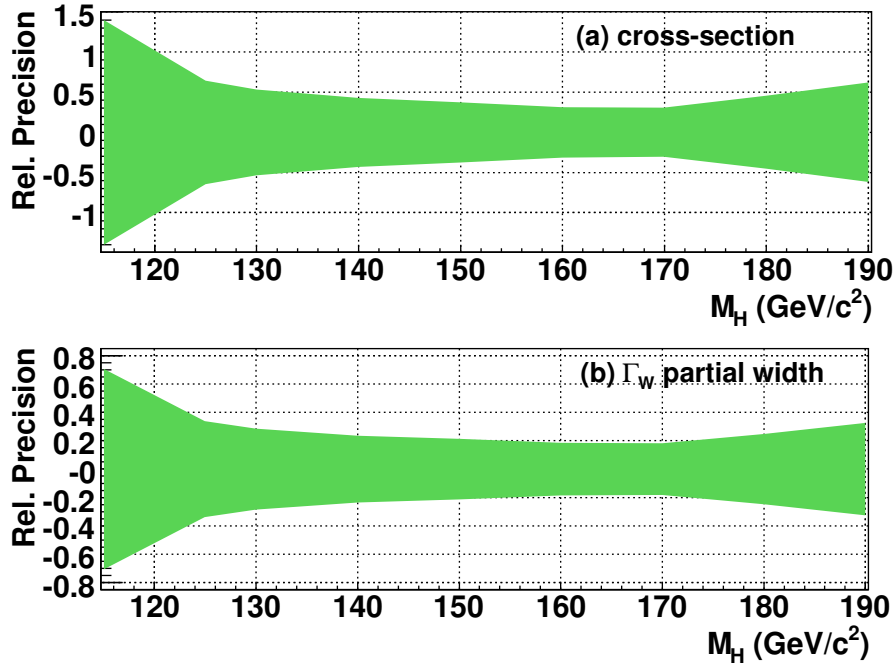
Figure 10.47: (a) Resolution on the product of cross-section and branching ratio into WW as a function of the Higgs boson mass, for an integrated luminosity of 100fb^{-1} . (b) Resolution on the \Gamma_W partial width as a function of the Higgs boson mass, for the same integrated luminosity.
