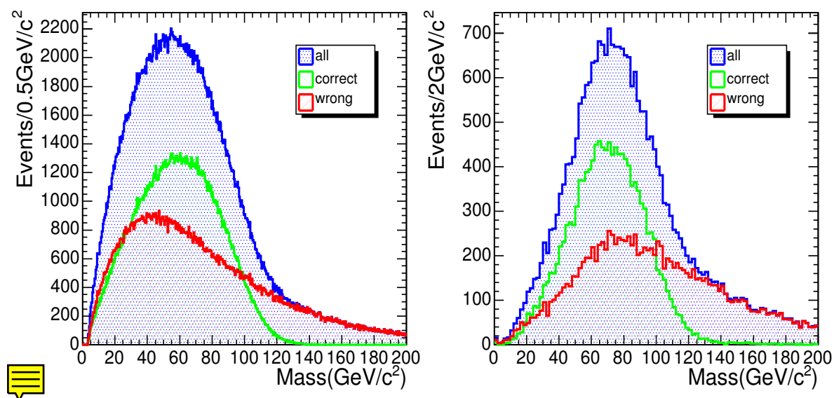
Figure 8.9: Three-lepton mass distribution for m_t = 175 \text{ GeV}/c^2 at generator level (left) and after detector simulation and reconstruction (right). In the pictures the components coming from correct and wrong lepton pairing - from both combinatorial and physics backgrounds - are shown.
