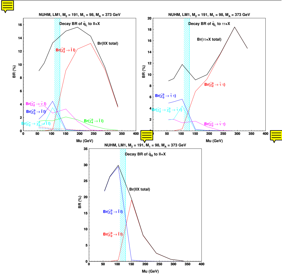
Figure 13.32: Decay branching ratios as a function of \mu for \tilde{q}_L into ll and \tau\tau and for \tilde{q}_R into ll at the test point LM1.
