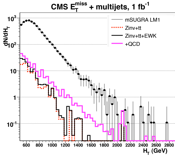
Figure 4.18: H_T LM1 signal and Standard Model background distributions.
