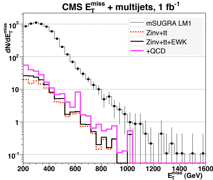
Figure 4.17: E_T^{\text{miss}} LM1 signal and Standard Model background distributions.
