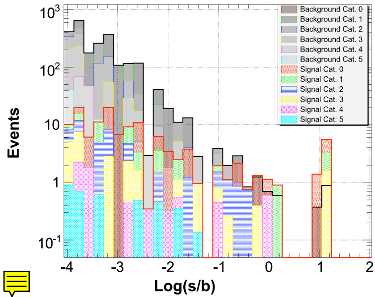
Figure 2.7: The final distribution of binned signal ( M_H=120 GeV) and background in \log(s/b) for an integrated luminosity of 7.7 \text{ fb}^{-1} .
