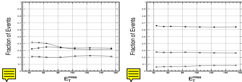
Figure 10.20: The fraction of events in different regions for the overall background (left) and VBF Higgs signal (right) as a function of E_T^{\text{miss}} cuts. Region A (close square), Region B (open square), and Region C (open circle).
