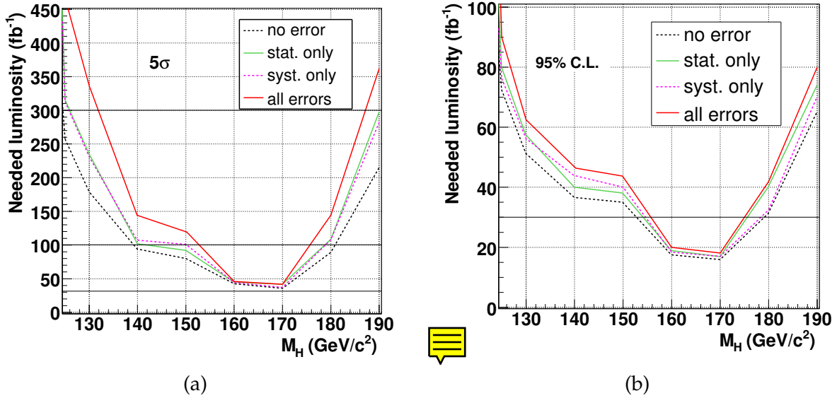
Figure 10.27: (a) Luminosity needed to obtain a 5\sigma significance using the likelihood-ratio method, with systematics only, Monte-Carlo statistical uncertainties only, or with both effects considered; (b) luminosity needed to exclude a Higgs boson at 95% C.L. if no excess is observed, using the same method.
