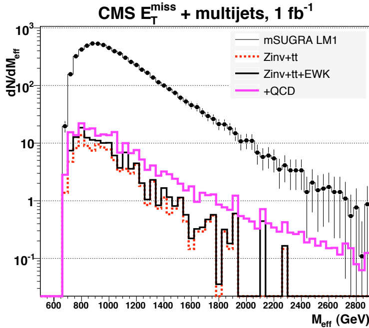
Figure 13.5: M_{\text{eff}} signal and background distribution in missing energy plus jets SUSY search.
