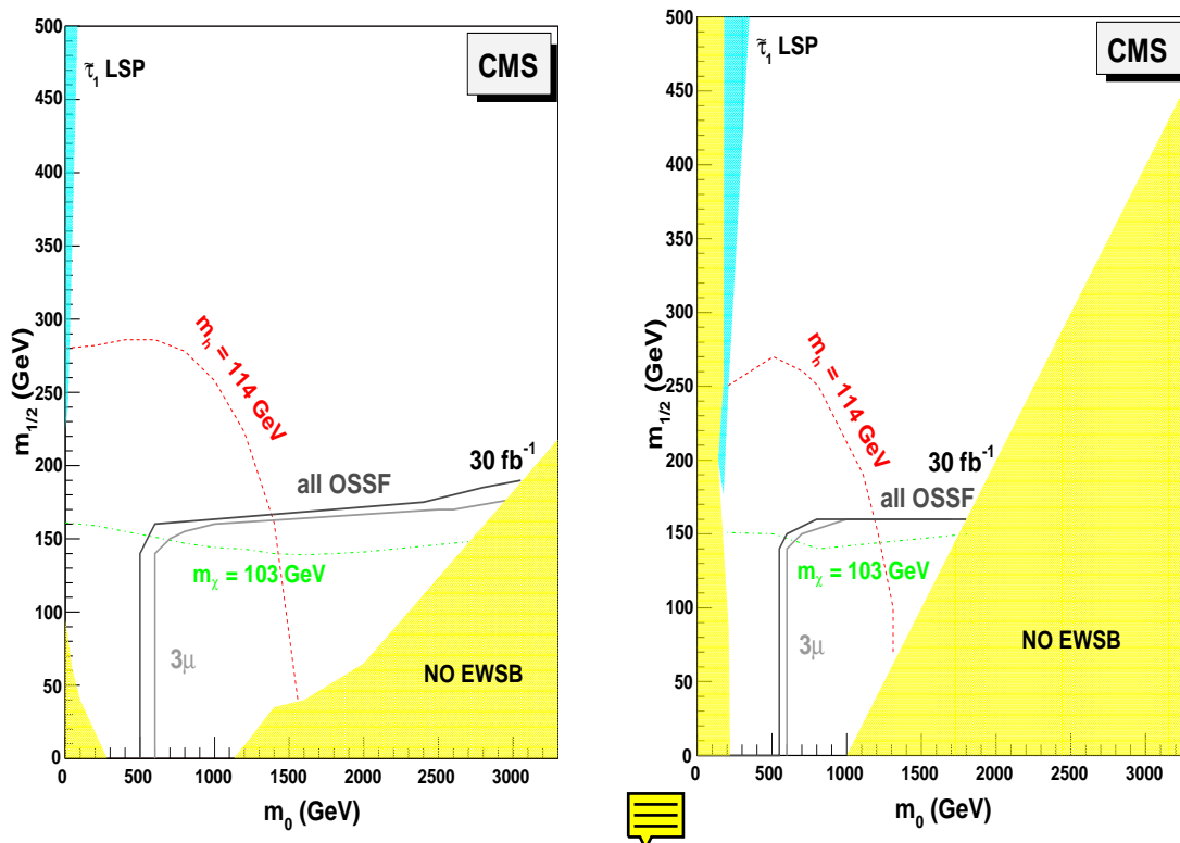
Figure 13.27: Discovery reach of trilepton from the pp \rightarrow \tilde{\chi}_2^0 \tilde{\chi}_1^\pm production at L_{int}=30 \text{ fb}^{-1} for all OSSF lepton combinations (dashed) and for the trimuon final state (solid) including systematic uncertainties from reconstruction.
