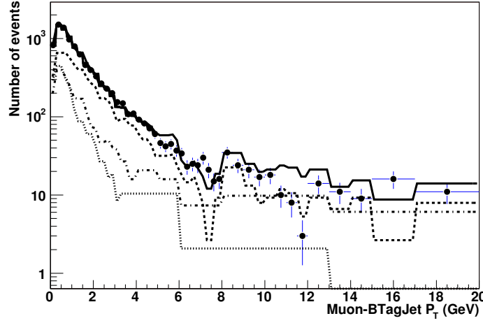
Figure 7.10: Fit of the muon p_T spectrum with respect to the closest b tagged jet. The sample of generated QCD events with “ p_T -hat” parameter in the range 230 < \hat{p}_T < 300 \text{ GeV}/c is tested. The contributions of tagged muons from b events (dashed curve), c events (dot-dashed curve) and light quark events (dotted curve) as defined by the fit are shown. The solid curve is the sum of the three contributions.
