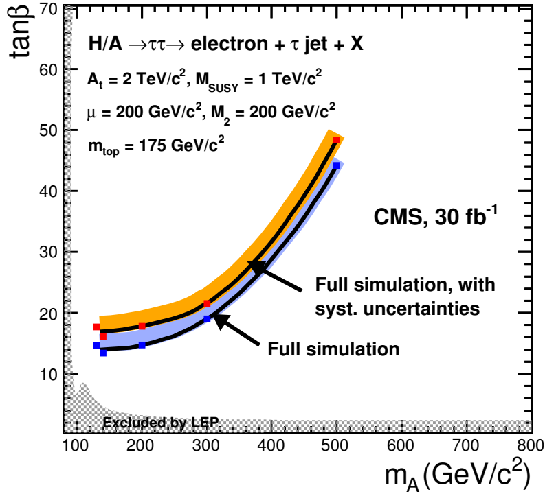
Figure 5.11: The 5\sigma discovery region in the M_A - \tan(\beta) plane with 30 \text{ fb}^{-1} of the integrated luminosity for the m_h^{\max} scenario. The lower (upper) curves was evaluated without (with) the effect of background systematics taken into account.
