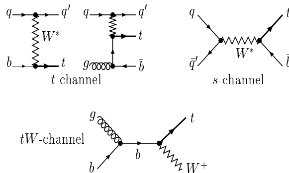
Figure 8.14: Feynman diagrams for the three channels of single top production.
