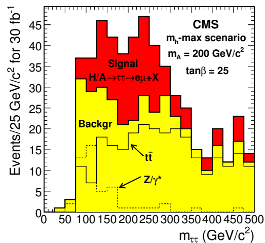
Figure 11.7: The \tau\tau reconstructed mass with 30 \text{ fb}^{-1} after all selections, but the mass window. The signal of M_A = 200 \text{ GeV}/c^2 and \tan\beta = 25 in the m_h^{\text{max}} scenario and the backgrounds are shown.
