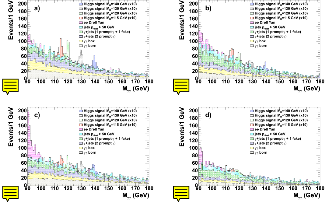
Figure 2.2: Invariant mass spectrum after the selection relative to the cut-based analysis with four categories defined in the text: barrel with large R_9 (a), barrel with small R_9 (b), endcaps with large R_9 (c) and endcaps with small R_9 (d). Events are normalized to an integrated luminosity of 1 \text{ fb}^{-1} and the Higgs signal, shown for different masses, is scaled by a factor 10.
