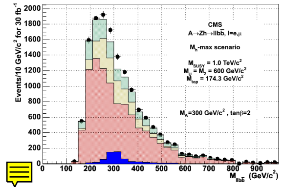
Figure 11.32: Distribution of M_{\ell^+\ell^-b\bar{b}} for signal and background after event selection for 30 \text{ fb}^{-1} of integrated luminosity. Red (dark gray), yellow (light gray) and green (medium gray) distributions represent the Zb\bar{b} , t\bar{t} and Z+\text{jets} backgrounds. Blue (black) distribution is the signal ( M_A=300, \tan\beta=2 ) and black dots the data (sum of the signal and the background).
