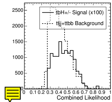
Figure 11.26: Distribution of the discriminator used to distinguish between signal 11.10 and background.
