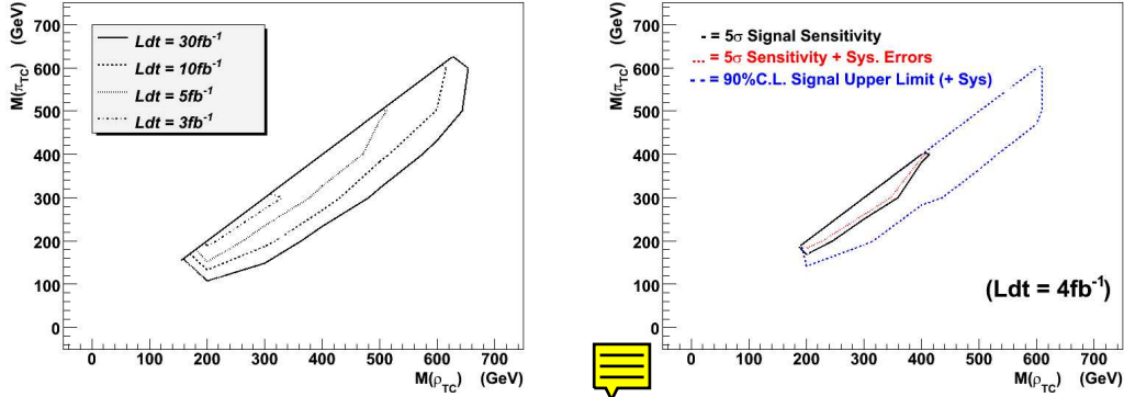
Figure 15.2: (a) Signal 5\sigma Sensitivity curves at various integrated luminosities; (b) sensitivity at \int Ldt = 4fb^{-1} : the dotted (resp. dashed) curve shows the sensitivity (resp. the 90% C.L. signal upper limit) after including systematic uncertainties.
