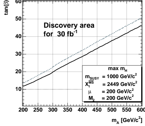
Figure 5.6: The 5\sigma discovery region in the M_A - \tan(\beta) plane with the 30 \text{ fb}^{-1} of the integrated luminosity for the m_h^{\text{max}} MSSM scenario. The regions are shown without (lower curve) and with (upper curve) the uncertainty on the background taken into account.
