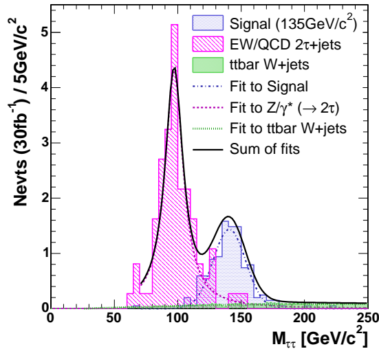
Figure 10.16: The invariant mass of two reconstructed \tau 's. The number of entries in each histogram is normalized to the expected number of events at an integrated luminosity of 30 \text{ fb}^{-1} .
