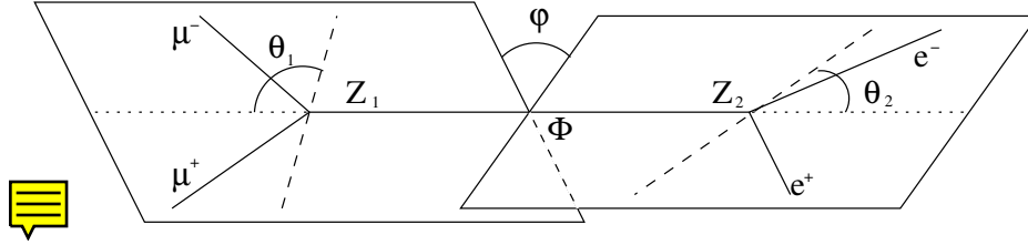
Figure 10.51: Definitions of the angles in the \Phi \rightarrow ZZ \rightarrow 2e2\mu process.
