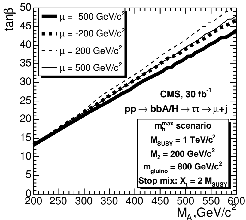
Figure 11.41: Variation of the 5\sigma discovery potential for the neutral Higgs bosons with the \tau\tau \rightarrow \mu + \text{jet} decay mode in the m_h^{\text{max}} scenario.
