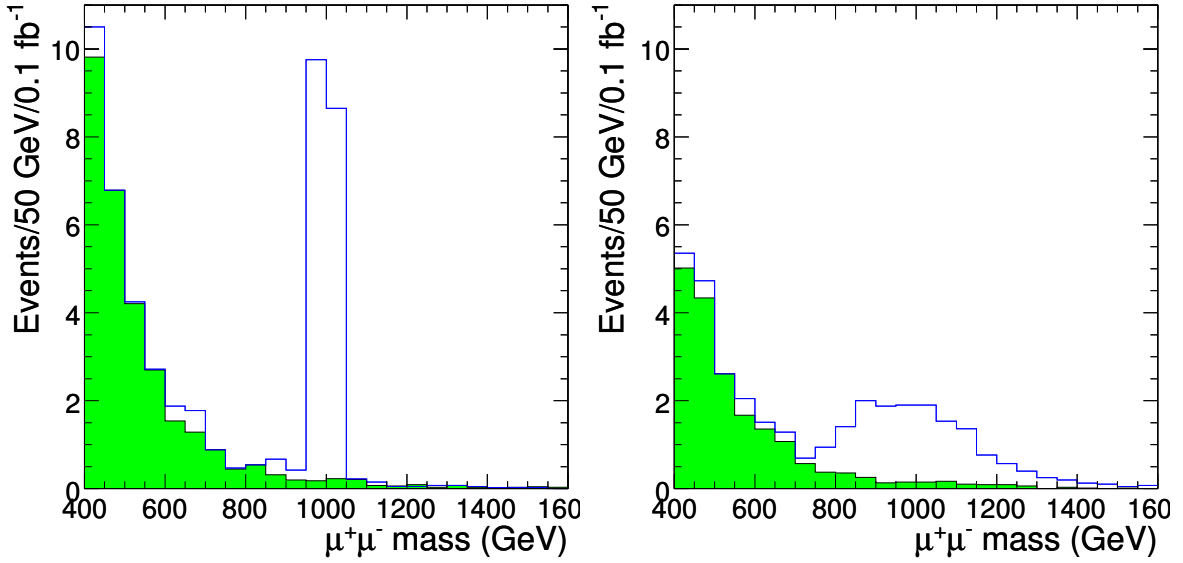
Figure 3.19: Histograms of the \mu^+\mu^- invariant mass for 1 TeV Z_\eta plus background (open histogram) and for background only (shaded histogram), at the event-generator level (left) and for events selected by the Level-1/HLT triggers and reconstructed assuming the “first data” misalignment scenario (right). The number of events per bin is normalized to an integrated luminosity of 0.1 \text{ fb}^{-1} .
