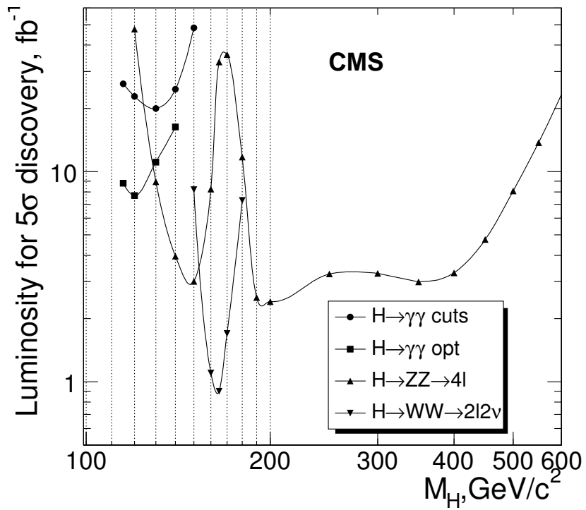
Figure 10.49: The integrated luminosity needed for the 5\sigma discovery of the inclusive Higgs boson production pp \rightarrow H + X with the Higgs boson decay modes H \rightarrow \gamma\gamma , H \rightarrow ZZ \rightarrow 4\ell , and H \rightarrow WW \rightarrow 2\ell 2\nu .
