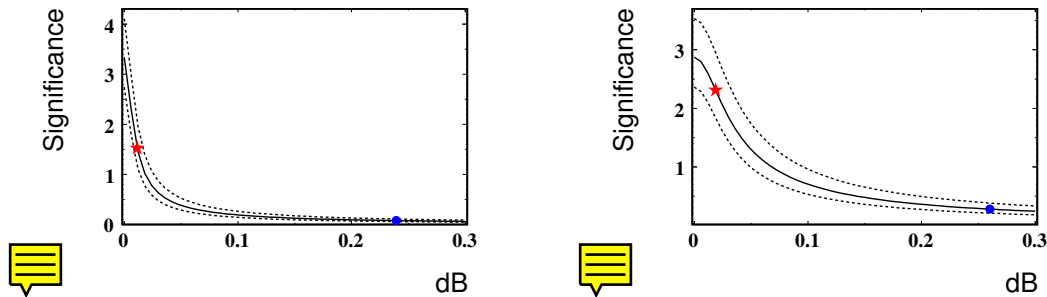
Figure 5.18: Expected range of combined significance (di-lepton + semi-leptonic + all-hadron) versus the total systematic uncertainty in background as a fraction of total background. Left: Results for the “loose” working points. Right: Results for the “tight” working points.
