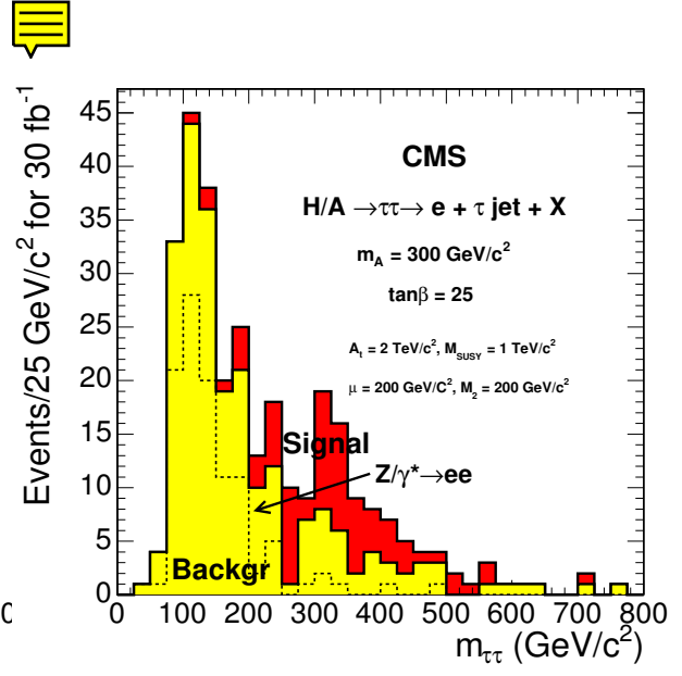
Figure 5.10: Reconstructed Higgs boson mass for the signal with M_A = 300 \text{ GeV}/c^2 and \tan\beta = 25 and for the total background for an integrated luminosity of 30 \text{ fb}^{-1} . The dashed line shows the sum of the Z/\gamma^* \rightarrow e^+e^- and b\bar{b}Z/\gamma^*e^+e^- backgrounds.
