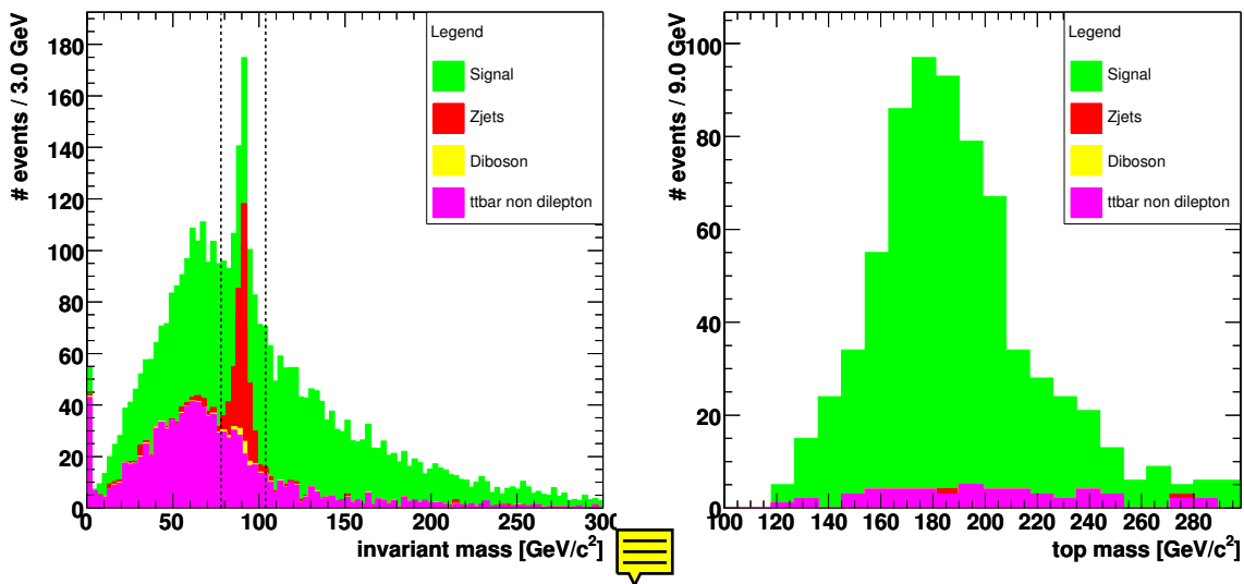
Figure 8.1: Left: Invariant mass of the two lepton candidates indicating the cut window to remove Z + \text{jets} events. Right: Most likely top mass after selection for 1 \text{ fb}^{-1} .
