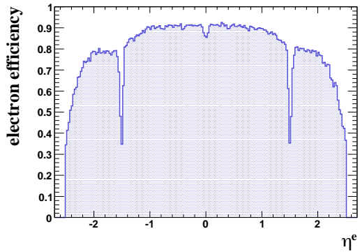
Figure 2.9: Electrons in SM Higgs boson 4e decay channel for m_H = 150 \text{ GeV}/c^2 ; a) transverse momentum of each of the four final state electrons; b) efficiency at pre-selection as a function of p_T^e ; c) efficiency at pre-selection as a function of \eta_e ; d) efficiency in the p_T^e versus \eta_e plane.
