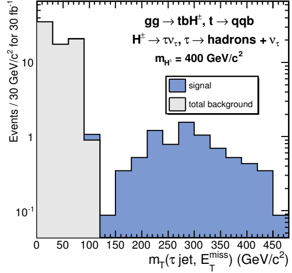
Figure 11.20: Transverse mass reconstructed from the \tau jet and missing transverse energy for the gg \rightarrow tbH^\pm, t \rightarrow bW, W^\mp \rightarrow jj signal (dark histogram) with m_{H^\pm} = 400 \text{ GeV}/c^2 , \tan\beta=30 and for the total background (light histogram) for an integrated luminosity of 30 \text{ fb}^{-1} .
