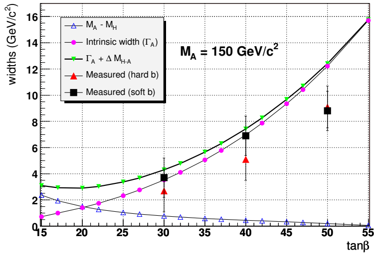
Figure 11.11: Compare between the expected effective Higgs boson width and the measured one as a function of \tan\beta for M_A = 150 \text{ GeV}
