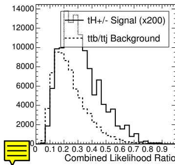
Figure 11.25: Distribution of the discriminator used to distinguish between signal 11.9 and background.
