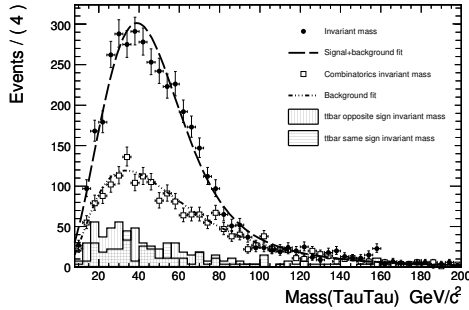
Figure 13.23: Di-tau invariant mass distributions.
