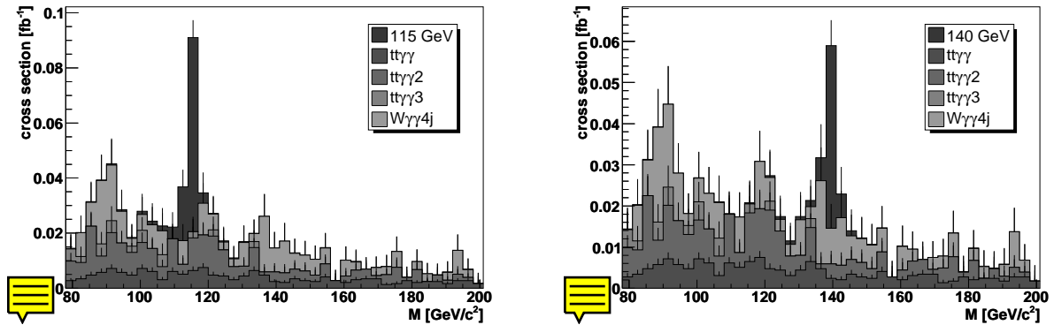
Figure 10.35: Invariant mass of the two Higgs photon candidates added to that of the sum of the surviving backgrounds after imposition of all selection requirements, for m_H = 115 GeV (left) and 140 GeV (right).
