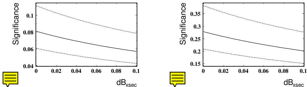
Figure 5.17: Expected range of combined significance (di-lepton + semi-leptonic + all-hadron, and includes the systematic uncertainties estimated in Section 5.3.6.1) versus an additional systematic uncertainty on the background cross-section as a fraction of total background. Left: Results for the “loose” working points. Right: Results for the “tight” working points.
