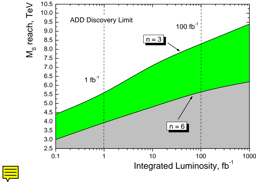
Figure 14.9: 5\sigma limit on M_S for the number of extra dimensions n = 3, 4, 5, 6 .
