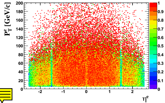
Figure 2.9: Electrons in SM Higgs boson 4e decay channel for m_H = 150 \text{ GeV}/c^2 ; a) transverse momentum of each of the four final state electrons; b) efficiency at pre-selection as a function of p_T^e ; c) efficiency at pre-selection as a function of \eta_e ; d) efficiency in the p_T^e versus \eta_e plane.
