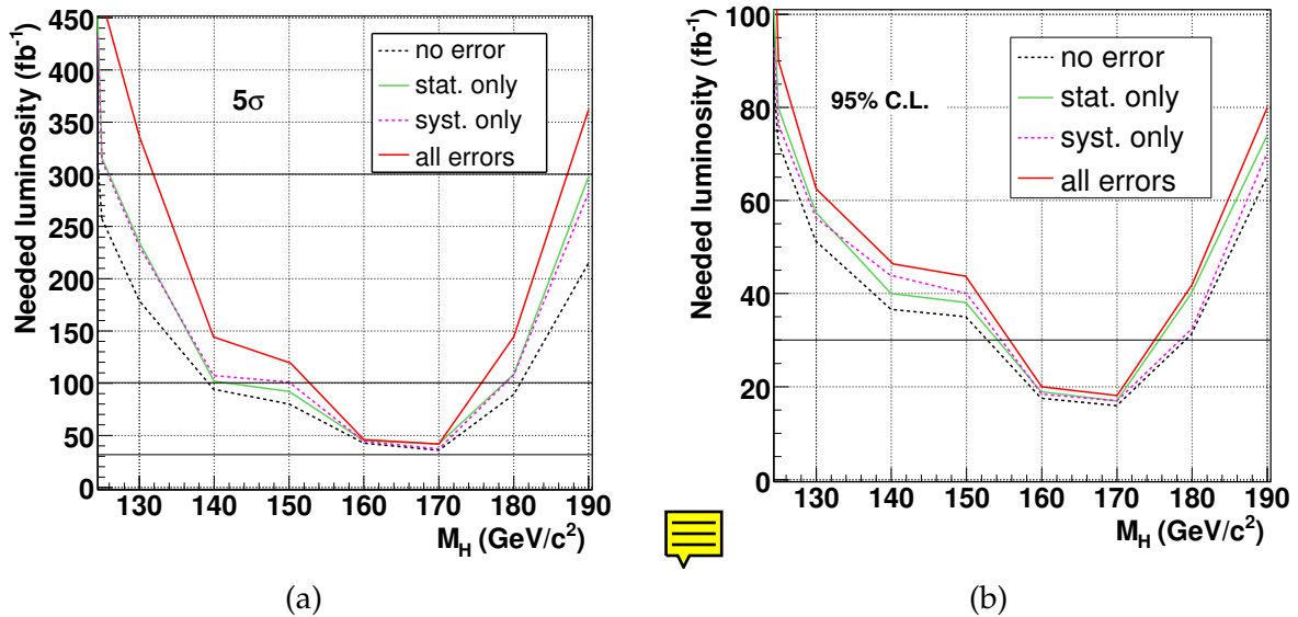
Figure 10.45: (a) Luminosity needed to obtain a 5\sigma significance using the likelihood-ratio method, with systematics only, Monte-Carlo statistical uncertainties only, or with both effects considered; (b) luminosity needed to exclude a Higgs boson at 95% C.L. if no excess is observed, using the same method.
