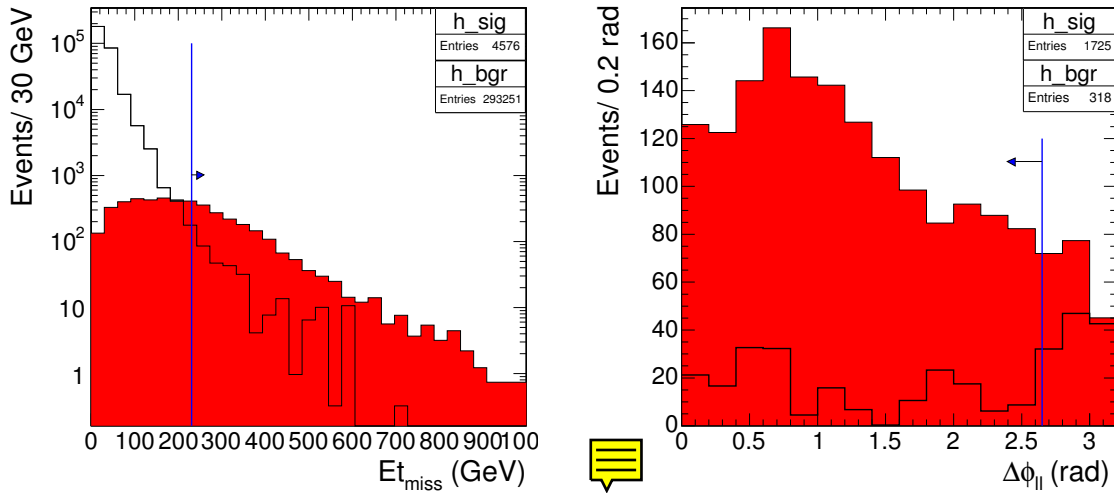
Figure 13.19: E_T^{\text{miss}} (a) and \Delta\phi between the two leptons (b) for background (black line) and signal (shaded) events. SUSY events not involving \tilde{\chi}_2^0 are considered signal. The vertical lines denote the E_T^{\text{miss}} and \Delta\phi requirements.
