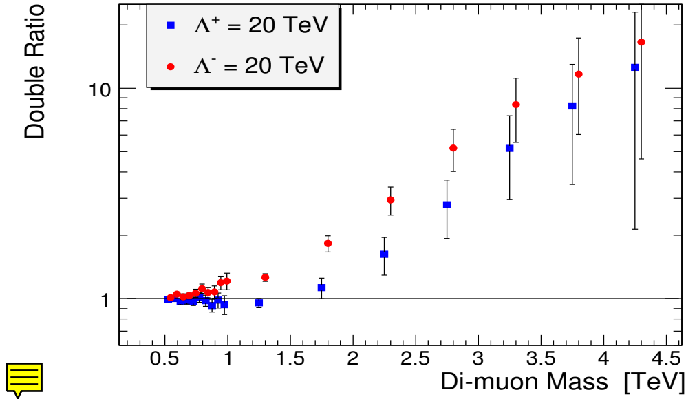
Figure 15.3: Double ratios for contact interactions in the di-muon channel, LL model, scale \Lambda = 20 TeV, positive and negative interference, and luminosity 100 \text{ fb}^{-1} . The errors shown are statistical.
