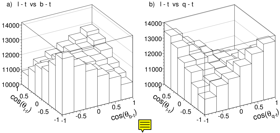
Figure 8.11: Double differential angular distributions obtained from the “analysis” sample, see text.
