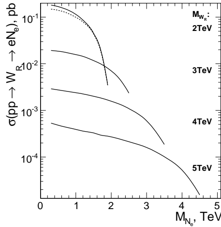
Figure 15.6: The dependence of the value \sigma(pp \rightarrow W_R) \cdot Br(W_R \rightarrow e^\pm N_e) on the heavy neutrino mass. For M_{W_R} = 2 \text{ TeV}/c^2 the same value in case of degenerated N masses is shown by the dashed line.
