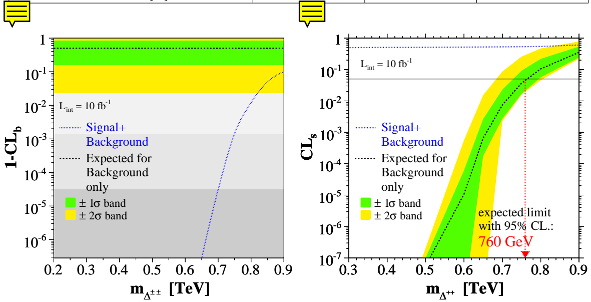
Figure 12.6: 1 - CL_b and CL_s as defined in the Log Likelihood Ratio Method after all selection cuts for an integrated luminosity of 10 \text{ fb}^{-1}
