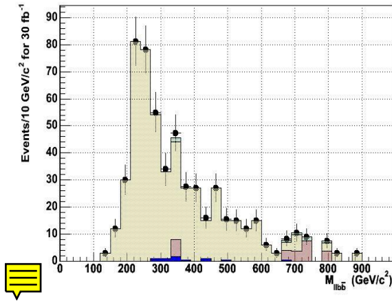
Figure 11.33: Distribution of M_{\ell+\ell-b\bar{b}} in the t\bar{t} background normalization region. Color code is as in Fig. 11.32
