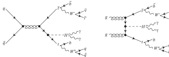
Figure 10.30: Typical diagrams for t\bar{t}H production with H \rightarrow \gamma\gamma and at least one charged lepton from the decay of a top or antitop quark.
