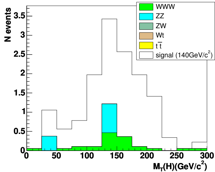
Figure 10.25: Reconstructed transverse mass from Equation 10.10 for a 140 GeV/c 2 Higgs boson and an integrated luminosity of 100 fb -1 .
