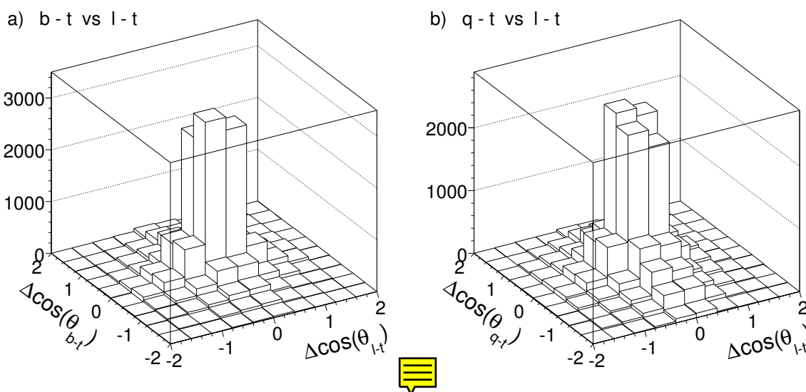
Figure 8.12: Selection quality: Difference between the generated and reconstructed cosine of the analysis angles in the b-ll-t and q-ll-t systems
