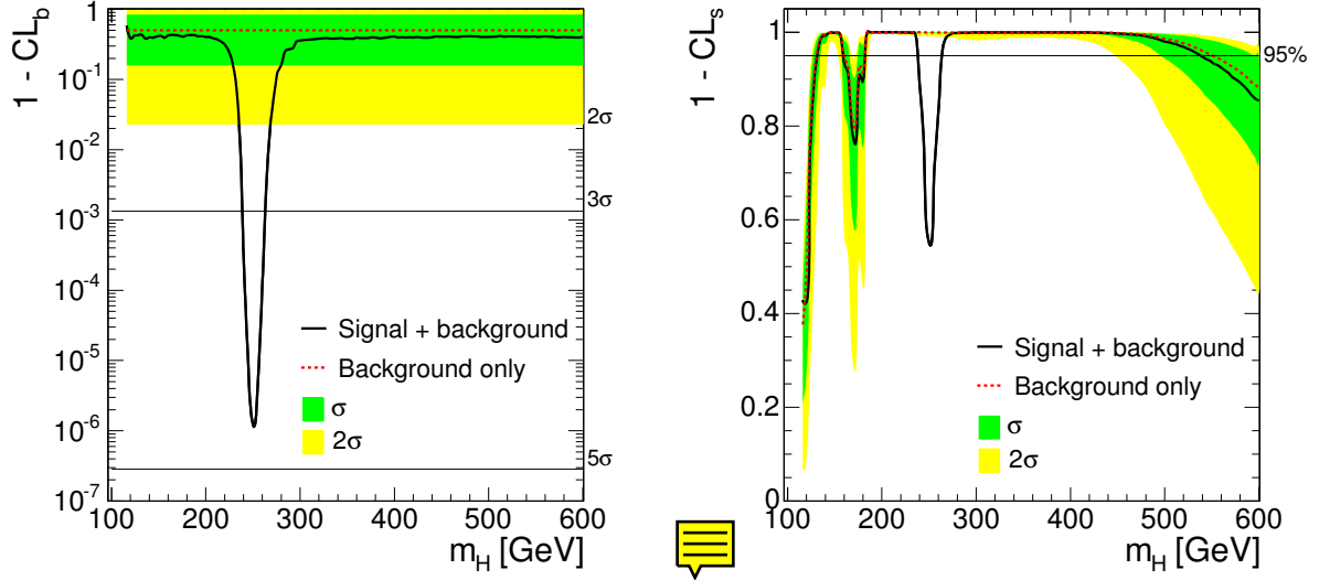
Figure 3.6: Mean values for 1 - CL_b (left) and 1 - CL_s (right) as a function of the Higgs boson mass hypothesis, assuming existence of Higgs boson at 250 GeV mass and for an integrated luminosity of 10 \text{ fb}^{-1} . The observation of the Higgs is just a little shy of the 5\sigma discovery (left). The mass points for which the curve 1 - CL_s is above 0.95 are excluded at 95% CL (right). The 1\sigma and 2\sigma bands on 1 - CL_b and 1 - CL_s , originating from the Poisson statistical fluctuations of the number of background events in each bin of the discriminant distribution, are also shown.
