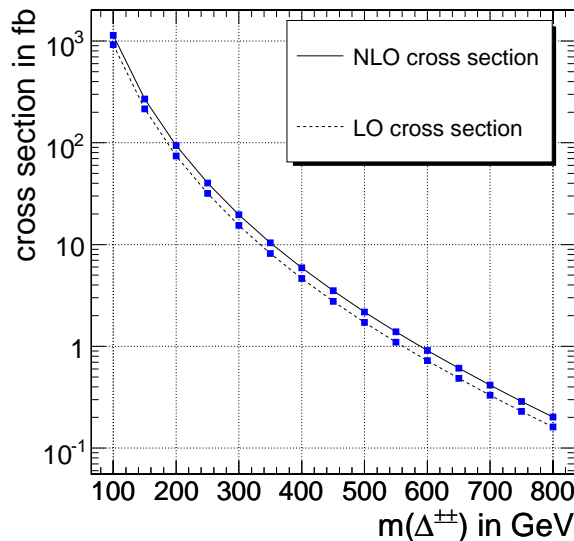
Figure 12.4: NLO Cross-section, for H^{++}H^{--} \rightarrow 4\mu .
