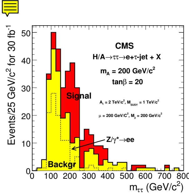
Figure 5.9: Reconstructed Higgs boson mass for the signal of M_A = 200 \text{ GeV}/c^2 and \tan\beta = 20 and for the total background for an integrated luminosity of 30 \text{ fb}^{-1} . The dashed line shows the sum of the Z/\gamma^* \rightarrow e^+e^- and b\bar{b}Z/\gamma^*e^+e^- backgrounds.
