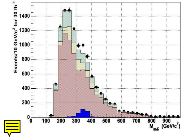
Figure 11.34: Distribution of M_{\ell+\ell-b\bar{b}} used in the Zb\bar{b} background estimation. Color code is as in Fig. 11.32
