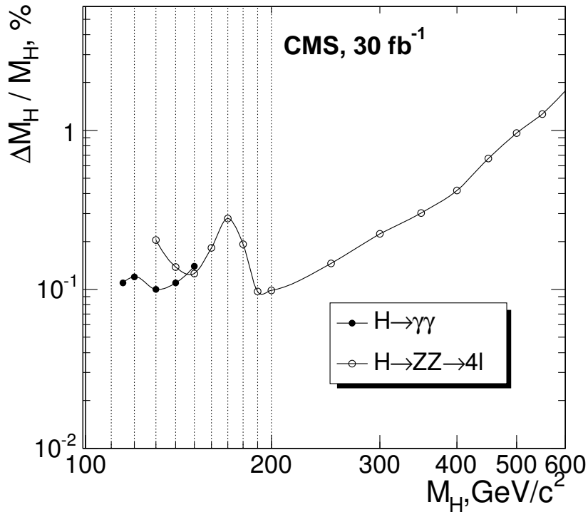
Figure 10.48: The statistical precision of the Higgs boson mass measurement for the 30 \text{ fb}^{-1} using inclusive Higgs boson production pp \rightarrow H + X and the H \rightarrow \gamma\gamma and H \rightarrow ZZ \rightarrow 4\ell decay modes.
