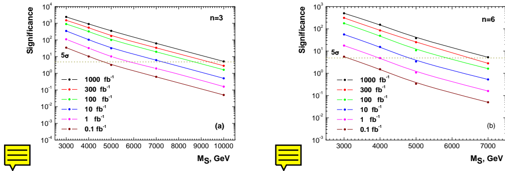
Figure 14.8: Significance as a function of M_S for (a) n = 3 and (b) n = 6 .
