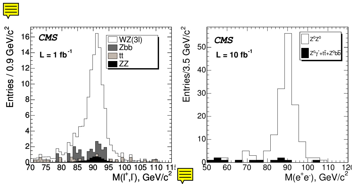
Figure 9.11: Left: Distribution of the mass of the Z^0 candidates for events retained by the W^\pm Z^0 selection, for an integrated luminosity of 1 \text{ fb}^{-1} . Right: Distribution of the mass of the Z^0 candidates, two entries per event, retained by the Z^0 Z^0 selection, for an integrated luminosity of 10 \text{ fb}^{-1} .
