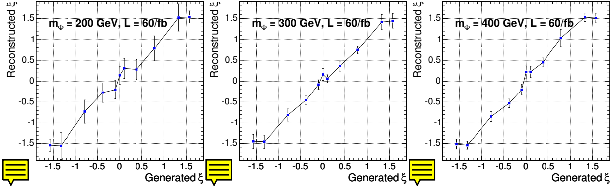
Figure 10.53: Reconstructed value of the parameter \xi as function of the generated value of the parameter \xi , for \mathcal{L}=60 \text{ fb}^{-1} , for Higgs boson mass m_\Phi=200, 300, 400 \text{ GeV} . Uncertainties correspond to one standard deviation.
