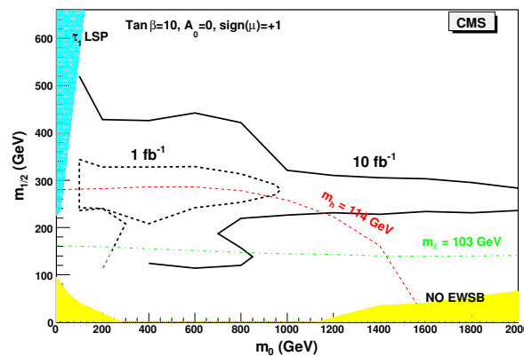
Figure 13.20: The 5 \sigma significance contours for 10 \text{ fb}^{-1} and 1 \text{ fb}^{-1} (dashed line) integrated luminosities and taking into account systematic uncertainties.
