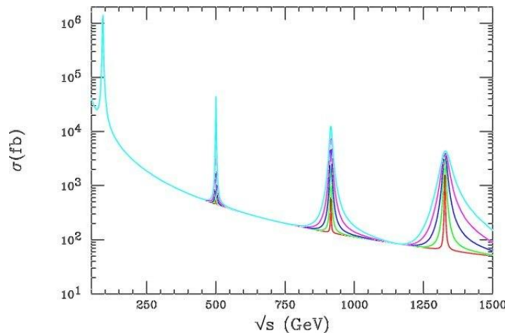
Figure 14.1: The cross section for e^+e^- \rightarrow \mu^+\mu^- including the exchange of KK gravitons in the RSI model. The narrowest resonances correspond to k/M = 0.05 , the widest to k/M = 0.1 . (taken from reference [687]).
