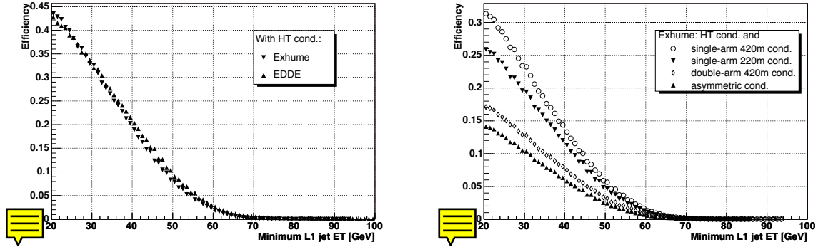
Figure E.1: L1 selection efficiency for pp \rightarrow pHp and H(120 \text{ GeV}/c^2) \rightarrow b\bar{b} as function of the E_T threshold value when at least 2 central L1 jets with E_T above threshold are required. All plots are for the non-pile-up case and the H_T condition has been applied. Left: Comparison between the EDDE and Exhume Monte Carlo generators, without applying any additional RP conditions. Right: Comparison of the effect of different RP conditions on the efficiency in the Exhume Monte Carlo sample.
