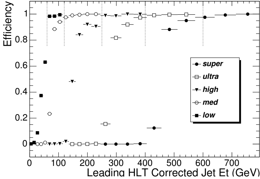
Figure E.4: The efficiency for passing the L1 jet trigger is shown as a function of HLT corrected jet E_T for each of the trigger paths shown in Table E.5. The L1 thresholds were chosen to give an efficiency of greater than 95% at the corresponding HLT threshold.
