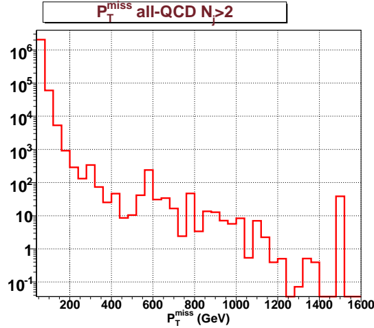
Figure 4.9: E_T^{\text{miss}} distribution in QCD 3-jet events.
