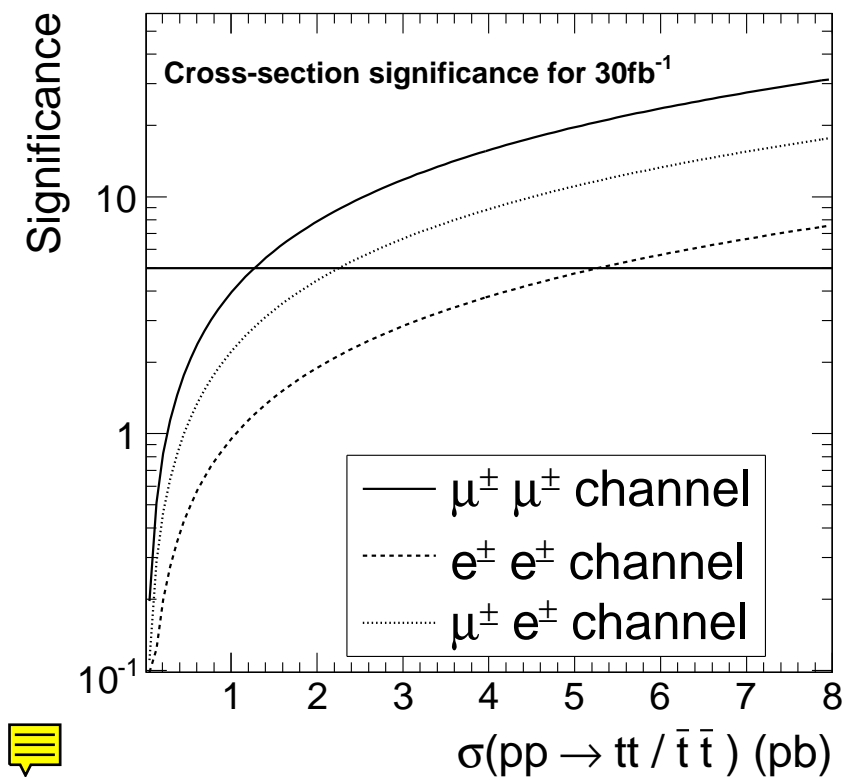
Figure 15.13: For an integrated luminosity of 30\text{fb}^{-1} the significance of the same-sign tt or \bar{t}\bar{t} excess above the Standard Model events is indicated as a function of the cross-section of the inclusive process pp \rightarrow tt/\bar{t}\bar{t} .
