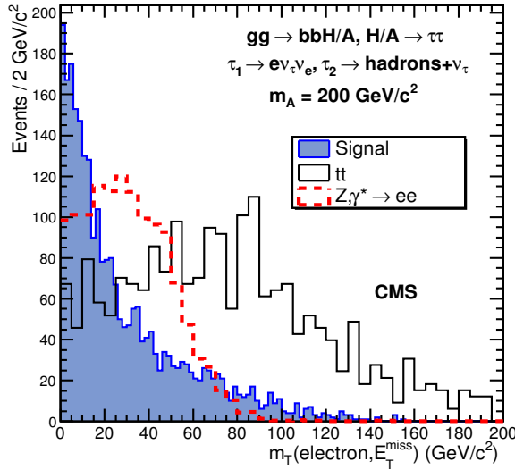
Figure 5.7: Distribution of transverse mass reconstructed from the electron and the missing transverse energy for the signal of M_A = 200 \text{ GeV}/c^2 and \tan\beta = 20 (filled histogram), for the t\bar{t} (solid line) and for the Z/\gamma^* \rightarrow e^+e^- (dashed line) background. Histogram normalization is arbitrary.
