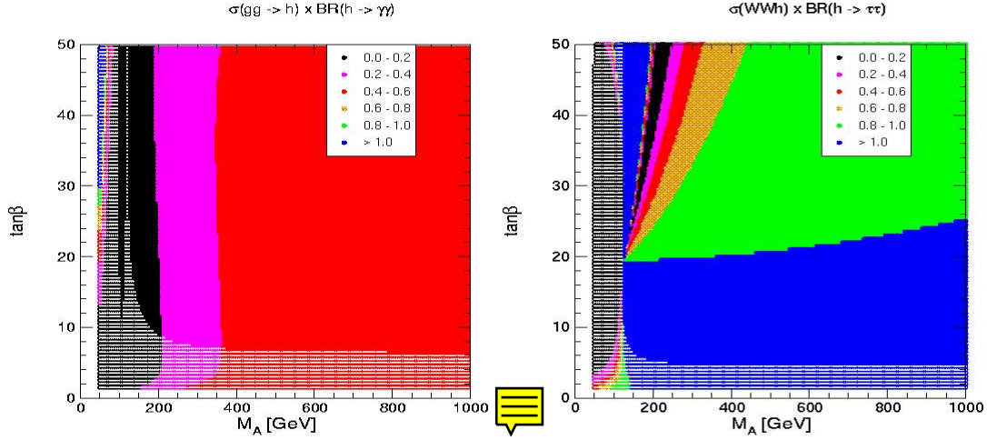
Figure 11.38: [\sigma \times \text{BR}]_{\text{MSSM}}/[\sigma \times \text{BR}]_{\text{SM}} is shown for the channels gg \rightarrow h \rightarrow \gamma\gamma in the gluophobic Higgs scenario (left plot) and WW \rightarrow h \rightarrow \tau^+\tau^- in the small \alpha_{\text{eff}} scenarios (right plot) in the M_A - \tan\beta -plane. The white-dotted area is excluded by LEP Higgs searches.
