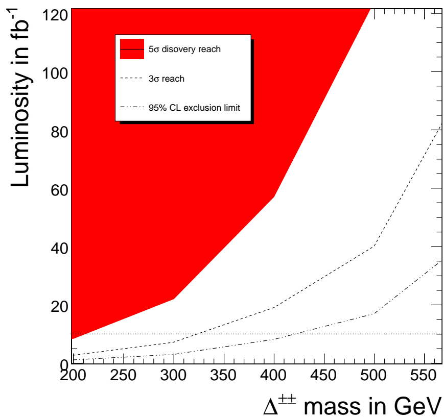
Figure 12.12: Mass reach in dependence to luminosity. 5\sigma , 3\sigma levels for discovery are given as well as 95% CL for exclusion if nothing is found by that time.
