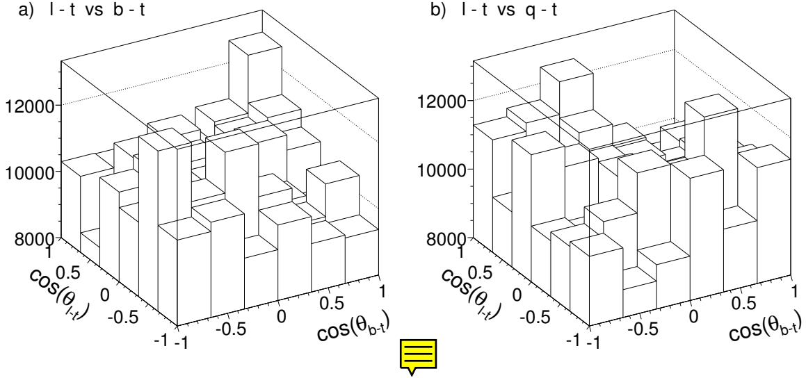
Figure 8.13: Background-subtracted and efficiency-corrected double-differential distribution of the cosine of the analysis angles in the b - ll - t and q - ll - t systems.
