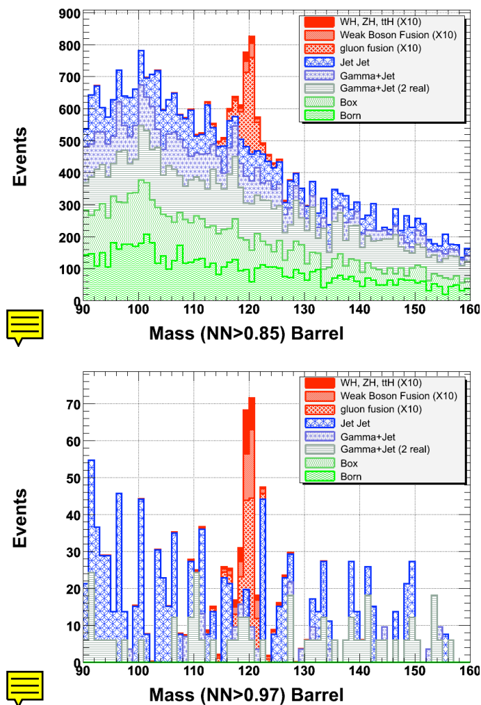
Figure 2.5: The di-photon mass distribution for each source for barrel events with kinematic neural net output greater than 0.85 (top) and 0.97 (bottom). The signal ( M_H=120 GeV) is multiplied by 10 for visibility.
