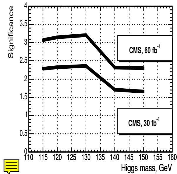
Figure 10.23: Significance vs Higgs boson invariant mass, normalized to 30 and 60 \text{ fb}^{-1} for instant luminosity 2 * 10^{33} \text{ cm}^{-2} \text{ s}^{-1}
