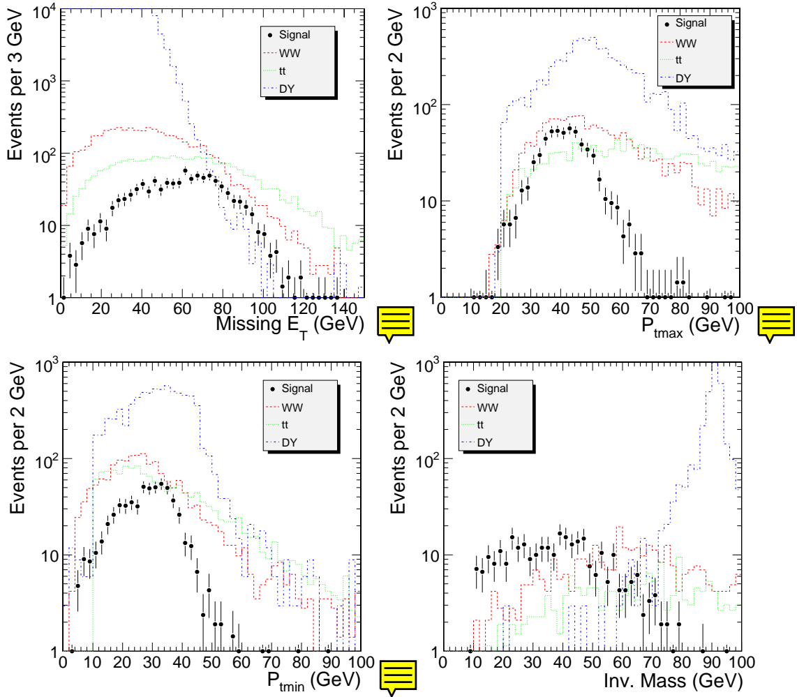
Figure 3.15: Distributions of the missing energy, transverse momentum and invariant mass for a luminosity of 10 \text{ fb}^{-1} following the cut list order.
