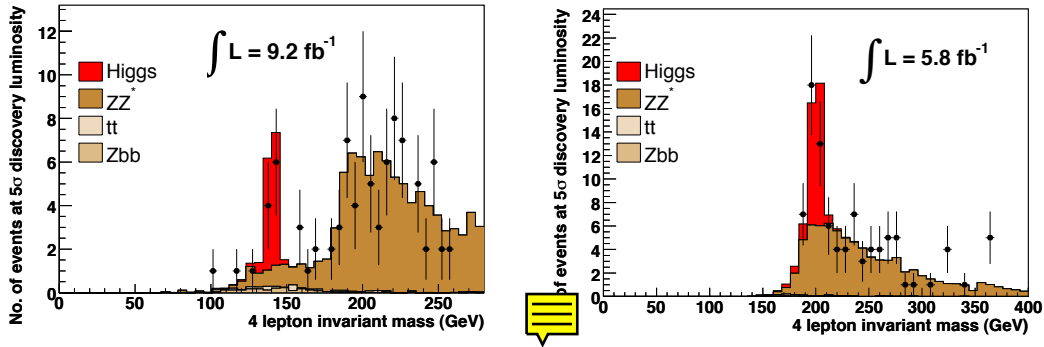
Figure 10.10: Number of expected events for signal and background for an integrated luminosity corresponding to a discovery significance of 5\sigma , for Higgs boson masses of 130 and 200 \text{GeV}/c^2 . The results of a simulated experiment are also shown to illustrate the statistical power of the analysis and the determination of the background normalization from data.
