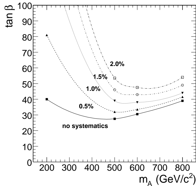
Figure 11.14: Two-sigma significance contour including some systematic error in the background calculation from Monte-Carlo shape. Statistics are for 60 \text{ fb}^{-1} .
