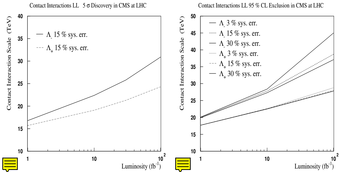
Figure 15.4: Five sigma discovery reach (left) and sensitivity at 95 % CL(right) for contact interactions in the di-muon channel for different luminosities and signs of the interference.
