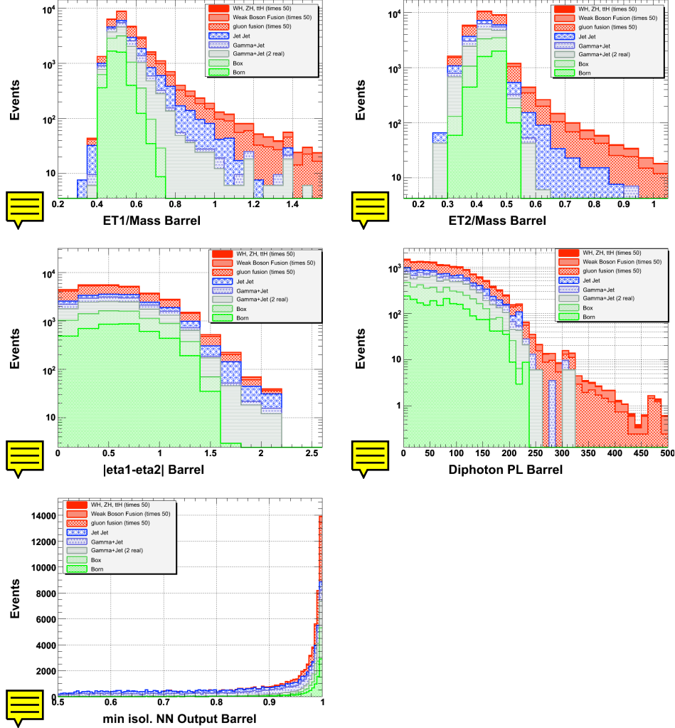
Figure 2.3: Distribution of the inputs to the neural network for signal and background sources. The signal is multiplied by 50 for visibility.
