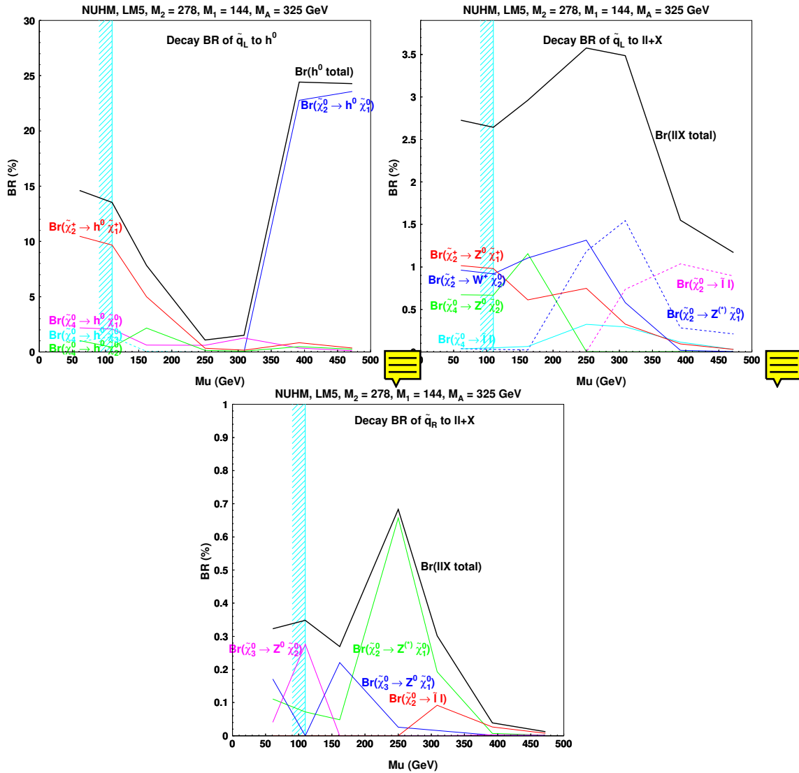
Figure 13.35: Decay branching ratios as a function of \mu for \tilde{q}_L into h^0 and ll and for \tilde{q}_R into ll at the test point LM5.
