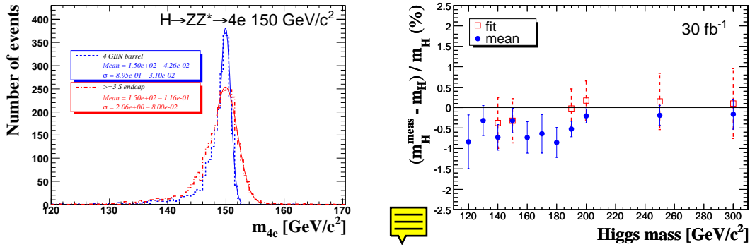
Figure 2.18: Mass measurements: (a) example case for two different event sub-samples differing by the pattern of the four reconstructed electrons; (b) relative errors as a function of the Higgs boson mass using the mean mass and the fitted mass as obtained for an integrated luminosity of 30 \text{ fb}^{-1} .
