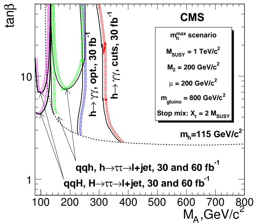
Figure 11.42: The 5\sigma discovery regions for the light, neutral Higgs boson h from the inclusive pp \rightarrow h+X production with the h \rightarrow \gamma\gamma decay and for the light and heavy scalar Higgs bosons, h and H , produced in the vector boson fusion qq \rightarrow qqh(H) with the h(H) \rightarrow \tau\tau \rightarrow \ell + \text{jet} decay.
