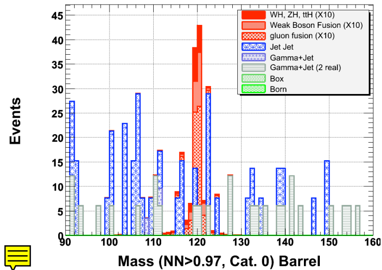
Figure 2.6: The Mass distribution for each source for barrel events with kinematic neural net output greater than 0.97 and R_9 > 0.948 . The signal for M_H=120 GeV is multiplied by a factor 10.
