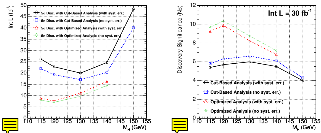
Figure 2.8: Integrated luminosity needed for a 5\sigma discovery (left) and discovery sensitivity with an integrated luminosity of 30 \text{ fb}^{-1} (right) with the optimized analysis. The results from the cut-based analysis in 12 categories are also shown for comparison.
