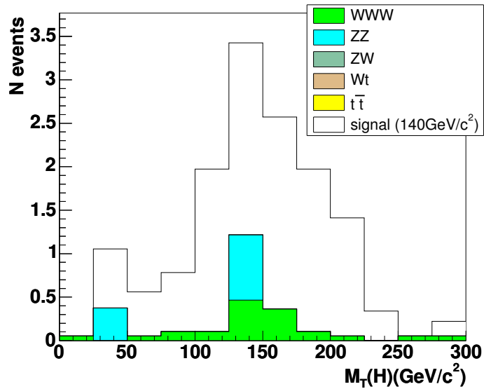
Figure 10.43: Reconstructed transverse mass from Equation 10.10 for a 140 GeV/c 2 Higgs boson and an integrated lumisonity of 100 fb -1 .
