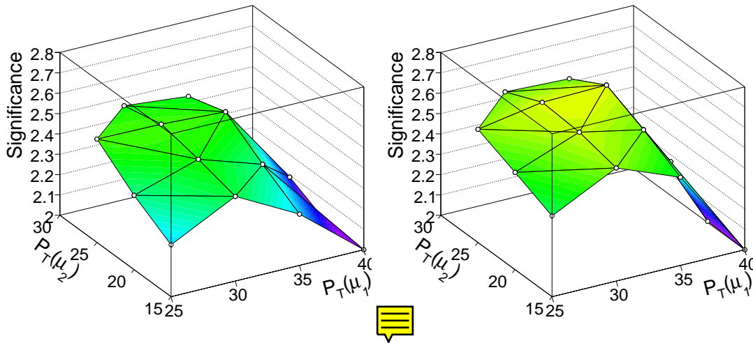
Figure 3.14: Significance as a function of P_T cuts for m_{\mu_1\mu_2} < 40 \text{ GeV} (left) and for m_{\mu_1\mu_2} < 50 \text{ GeV} (right) with L = 1 \text{ fb}^{-1} and \text{syst. err.} = 10\%
