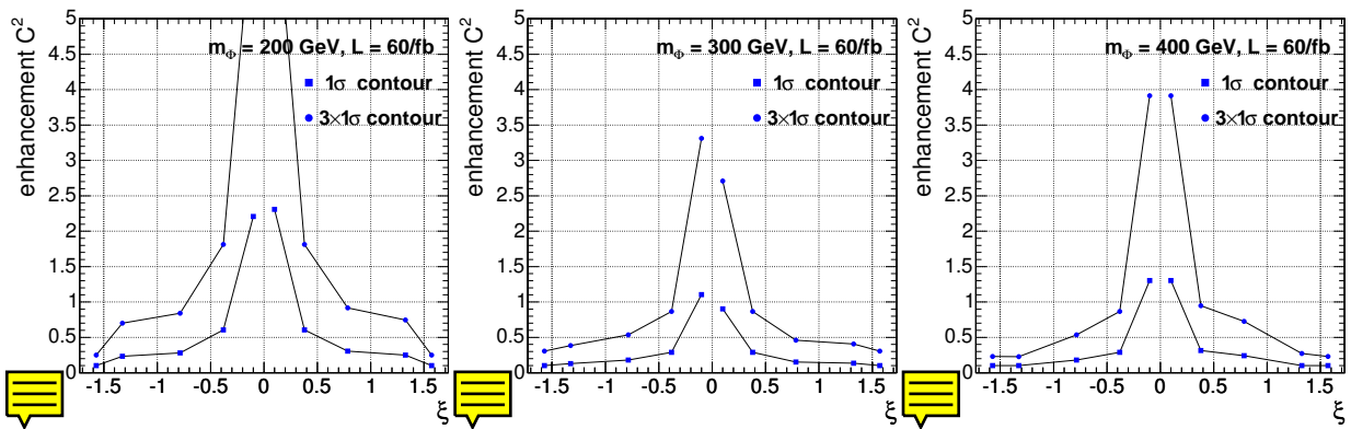
Figure 10.54: Exclusion contours for scalar Higgs boson as a function of the enhancement factor C^2 for the Higgs boson masses m_\Phi=200, 300, 400 GeV (from left to right). The excluded area lies above curves. Results were obtained for 60 \text{ fb}^{-1} .
