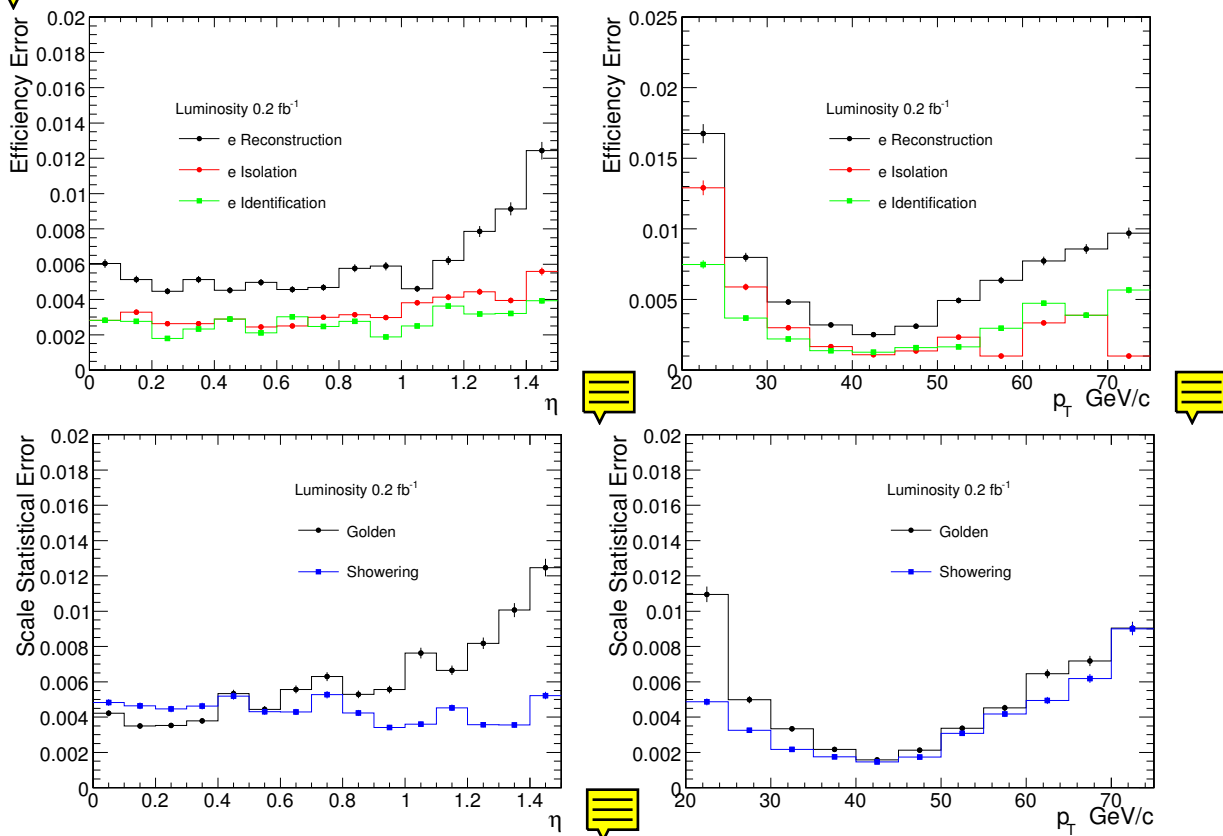
Figure 2.15: Control of experimental uncertainties using SM data; uncertainties on measurements of electron reconstruction, isolation and identification as a function of (a) \eta and (b) p_T ; uncertainties on measuring the energy scale for golden and showering electrons as a function of (c) \eta and (d) p_T .
