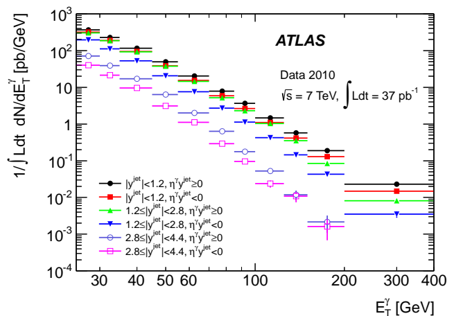
FIG. 1. Transverse energy distribution of photon candidates in photon + jet events selected in the 2010 ATLAS data, before background subtraction. The distribution is normalized by the integrated luminosity and the transverse energy bin width. Events with E_T^\gamma \leq 45 \text{ GeV} have been collected with the (prescaled) 20 GeV photon trigger. Events with E_T^\gamma > 45 \text{ GeV} have been collected with the (unprescaled) 40 GeV photon trigger.
